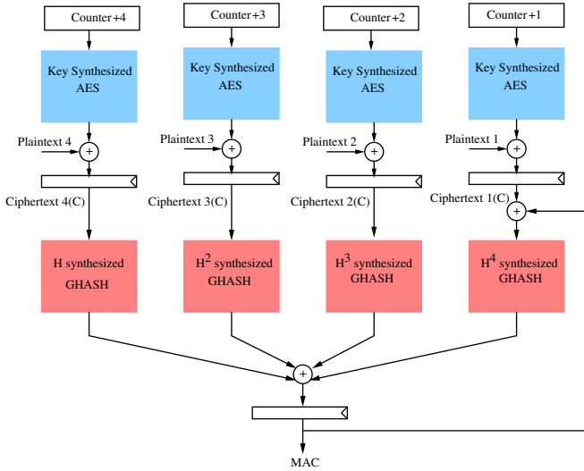
Figure 5. Presented 4-parallel AES-GCM using key-synthesized method
