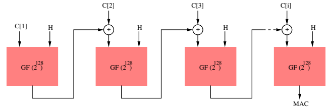
Figure 1. GHASH operation
