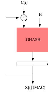
Figure 3. GHASH operation
