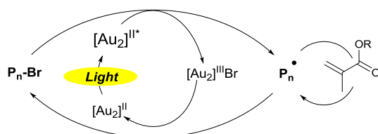
Scheme 3 Proposed mechanism for photo-ATRP of (meth)acrylates using [Au_2(\mu\text{-dppm})_2]Cl_2 as a photocatalyst.
