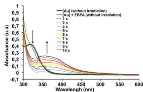
Figure 2 Steady state photolysis of 1 and 2 in dichloromethane upon exposure to the Xe-Hg under air at different irradiation times (from t = 0 to 10 s). 1/2 :
