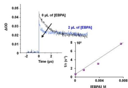
Figure 1 Laser flash photolysis. Decay of the [\text{1}]^{\text{II}*} signal at 390 nm in dichloromethane with increasing concentrations of 2 . The arrow shows that the \text{Au}_2^{\text{II}*} lifetime decreases as the concentration of 2 increases (from 0 to 7.6 \cdot 10^{-3} \text{ M} ). \Delta\text{OD} is the change in optical density associated with the light excitation ( \lambda = 355 \text{ nm} ).
