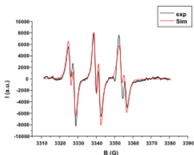
Figure 3. ESR spin trapping (PBN) spectrum. [\text{PBN}] = 7.90 \cdot 10^{-4} \text{ M} , [\mathbf{1}] = 1.57 \cdot 10^{-4} \text{ M} , [\mathbf{2}] = 1.91 \cdot 10^{-3} \text{ M} in 1.5 mL of DCM/ tert -butylbenzene 1:2.
