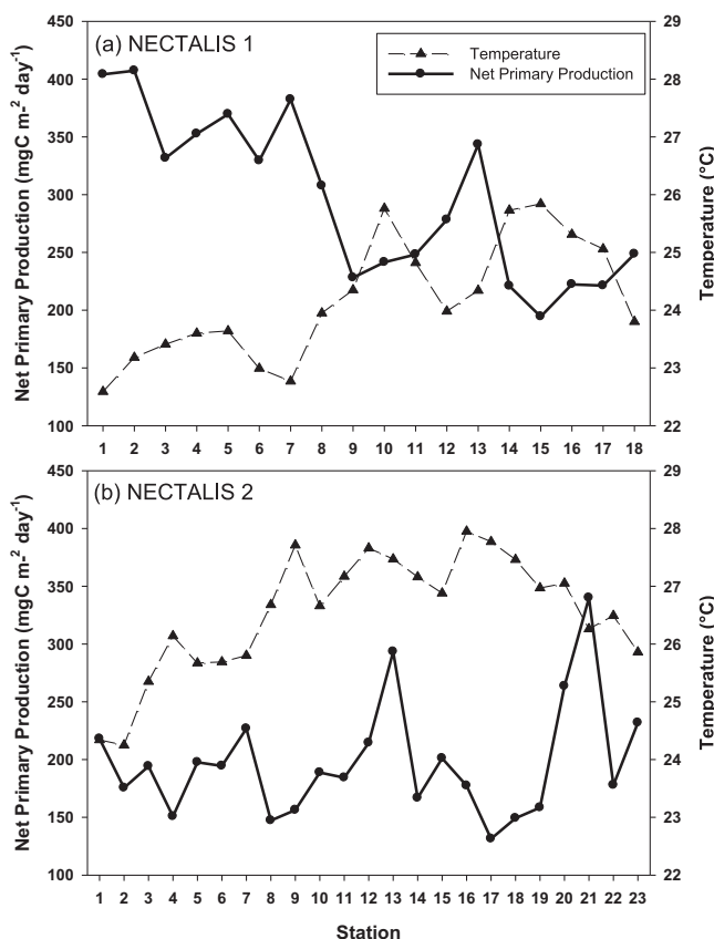
Figure 5. Satellite-derived sea surface temperature (SST) and net primary production (NPP) during the Nectalis cruises.
