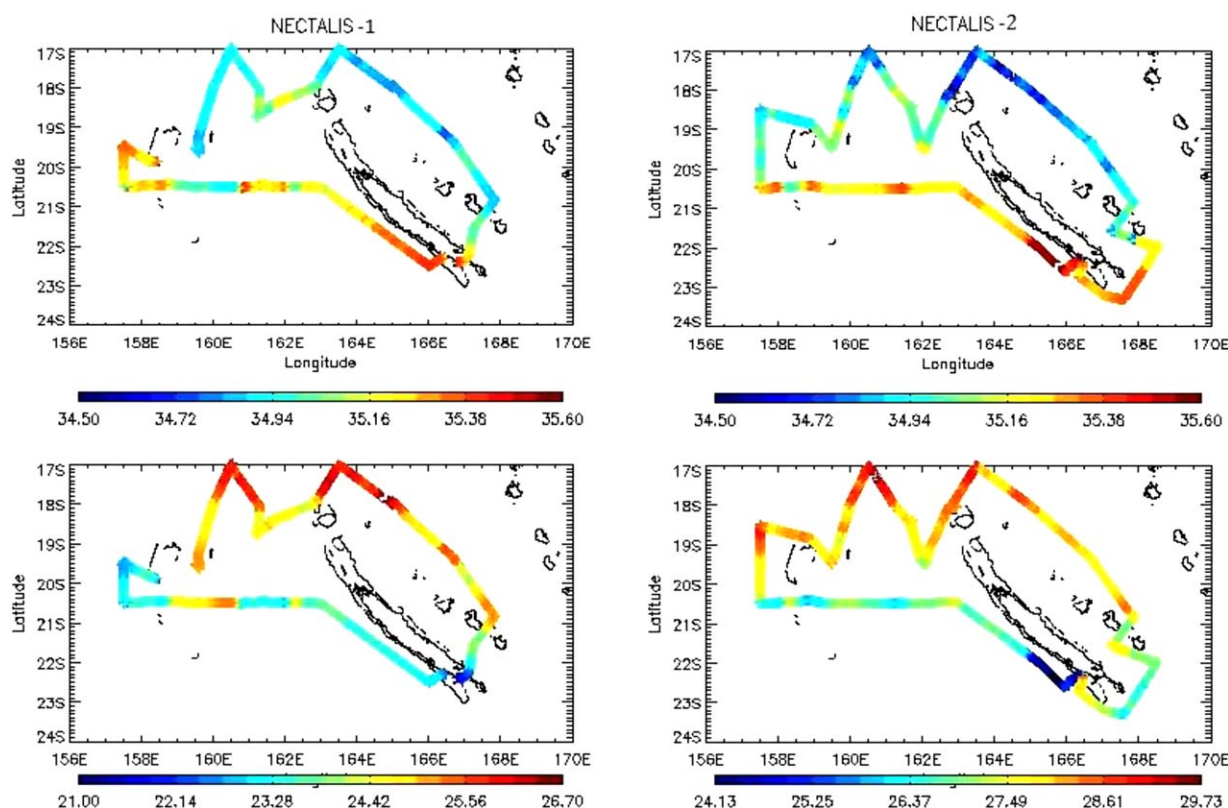
Figure 2. (top) Sea surface salinity SSS and (bottom) sea surface temperature SST ( ^{\circ}\text{C} ) from ship sensors during (left) Nectalis-1 and (right) Nectalis-2.
