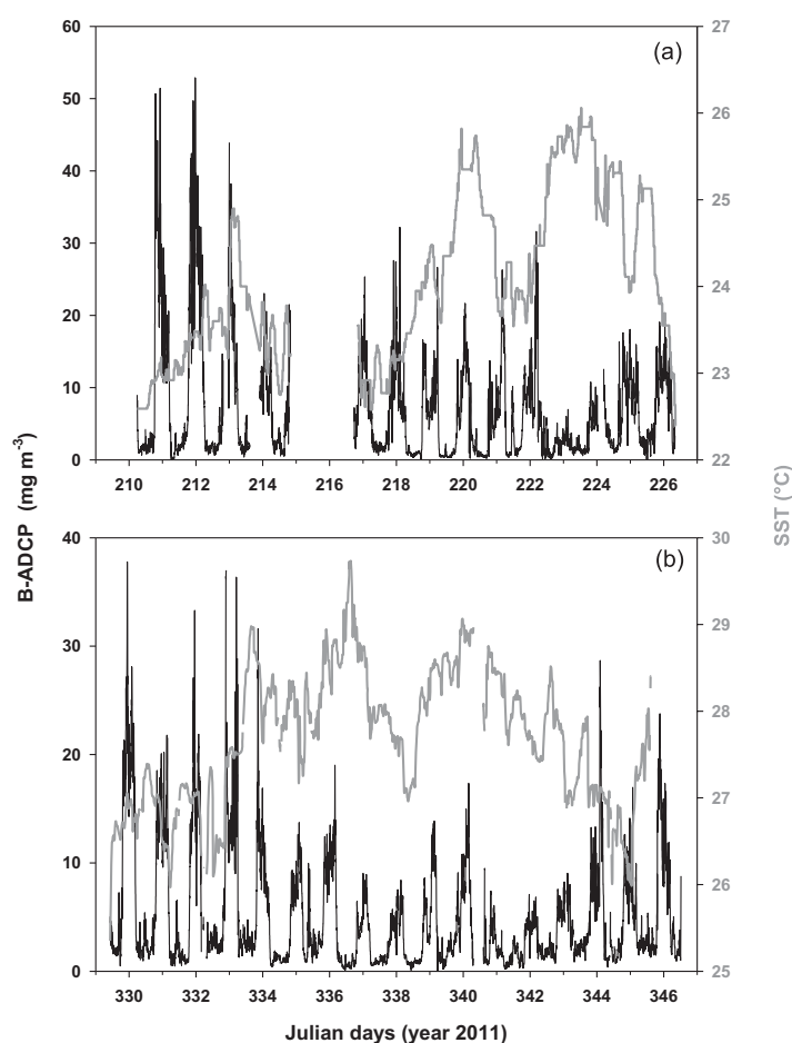
Figure 10. Depth integrated (16–104 m) zooplankton biomass (black lines) estimated from ADCP ( B_{ADCP} ) and sea surface temperature (SST - gray lines) during (a) Nectalis-1 and (b) Nectalis-2.
