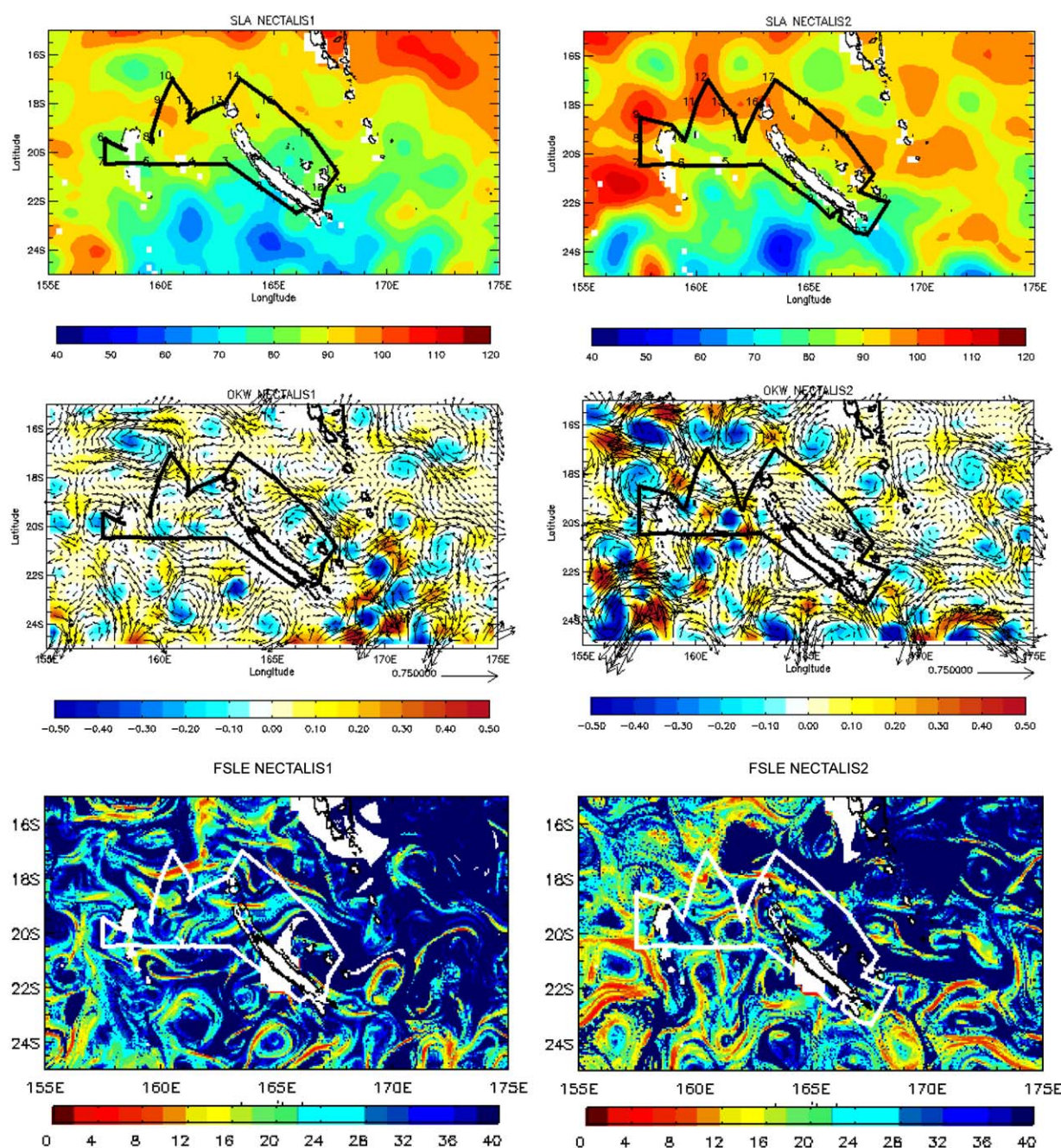
Figure 4. Contours of (top) sea level anomalies (SLA, color scale in cm), (middle) eddy depiction index Okubo-Weiß parameter (OKW, color scale in \text{day}^{-2} ) with an overlay of satellite-derived surface current vectors. SLA and OKW contours are adapted from Menkes et al. [2014]. (bottom) Mean FSLE during the Nectalis cruises, color scale in \text{day}^{-1} . (left) Nectalis-1 and (right) Nectalis-2. Cruise tracks are plotted as black solid lines in top and middle rows and as white solid lines in bottom row.
