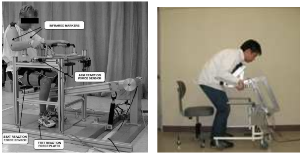
(a) FES Supported sit-to-stand rehabilitation robot (b) Standing Assistance System robot
