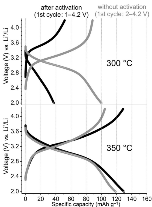
Figure 4. Discharge and charge curves obtained for \text{FeF}_{2.2}(\text{OH})_{0.8-x}\text{O}_{x/2}\square_{x/2} electrodes prepared at 300 and 350 °C, without (grey) and with (black) activation of the electrode down to 1 V. Cells were cycled under 50 \text{ mA g}^{-1} within the voltage window of 2–4.2 V.
