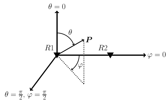
Figure 1. Spherical reference frame used throughout this study. The origin is placed at the location of receiver 1 ( R1 ), while receiver 2 ( R2 ) lies on the \varphi = 0, \theta = \pi/2 axis. The distance between the origin and a point P is denoted r .
