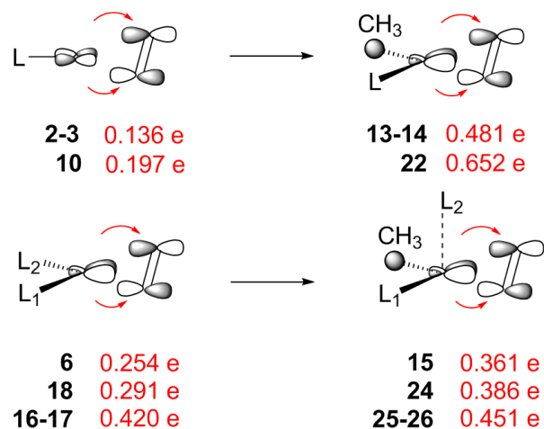
Fig. 5 Effect of additional alkyl group on the back-donation: in the case of monodentate (Me ( 10 and 22 ) and NHC ( [2,3] and [13,14] )) and bidentate ligands (BINAP, ( 6,15 ), DiPPAM, ( 18, 24 ) alkoxy-NHC [16,17] and 85 [25,26] ). The [a, b] notation refers to the average values for the two complexes.
