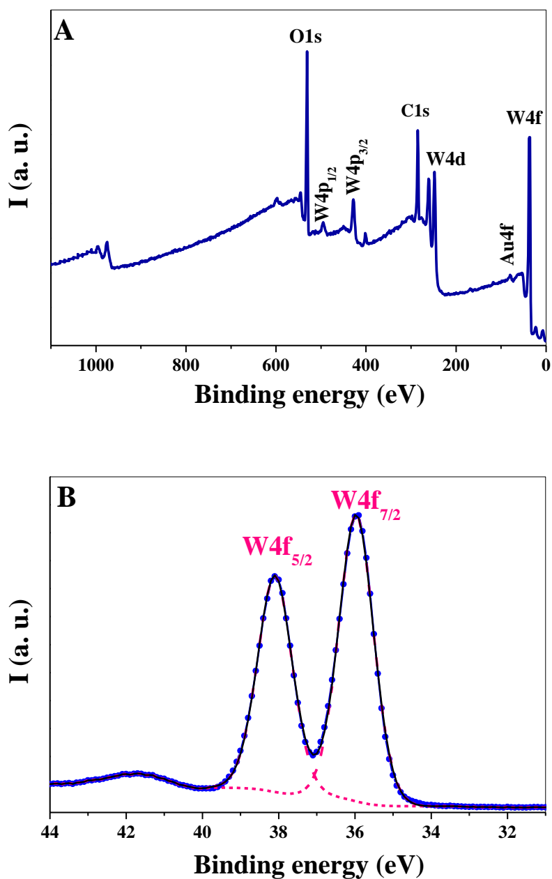
Fig. 4 X-ray Photoelectron Spectroscopy (XPS) survey spectrum (A) and the corresponding W 4f core level spectrum (B) of as-prepared dense WO 3 film electro synthesized at -0.5 V vs Ag/AgCl for 20 min.
