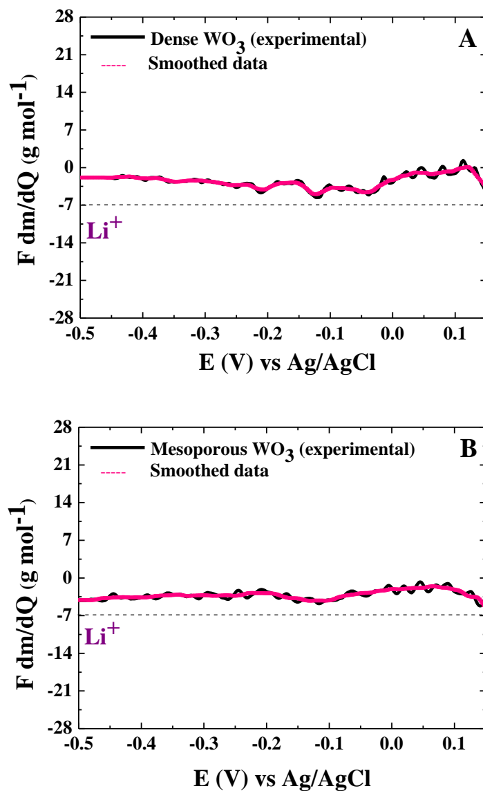
Fig. 6 F \times \frac{\Delta m}{\Delta q} values corresponding to the average molecular weight of the species involved in the charge compensation as a function of the potential for a dense (A) and a mesoporous (B) \text{WO}_3 film cycled in 0.5 M aqueous \text{LiClO}_4 solutions (obtained from the reduction branch of the EQCM results at a scan rate of 50 \text{ mV s}^{-1} ).
