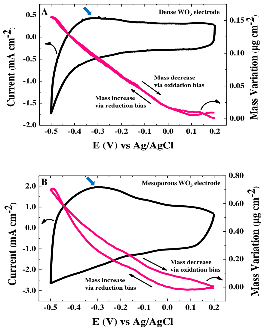
Fig. 5 Cyclic voltammograms and mass responses obtained simultaneously during the electrochromic response of (A) dense and (B) mesoporous WO 3 thin films deposited on the gold electrode of the quartz resonator. Measurements are in 0.5M aqueous solution of LiClO 4 with a scan rate of 50 mV s -1 .
