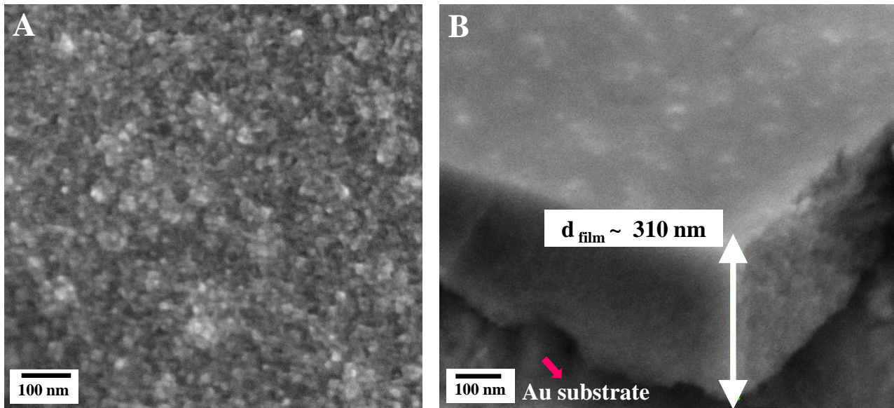
Fig. 2 FEG-SEM images showing the top view (A) and the cross-section (B) of an as deposited dense \text{WO}_3 thin film (electrodeposited on the Au electrode of a quartz resonator at -0.5 V vs Ag/AgCl during 20 min).
