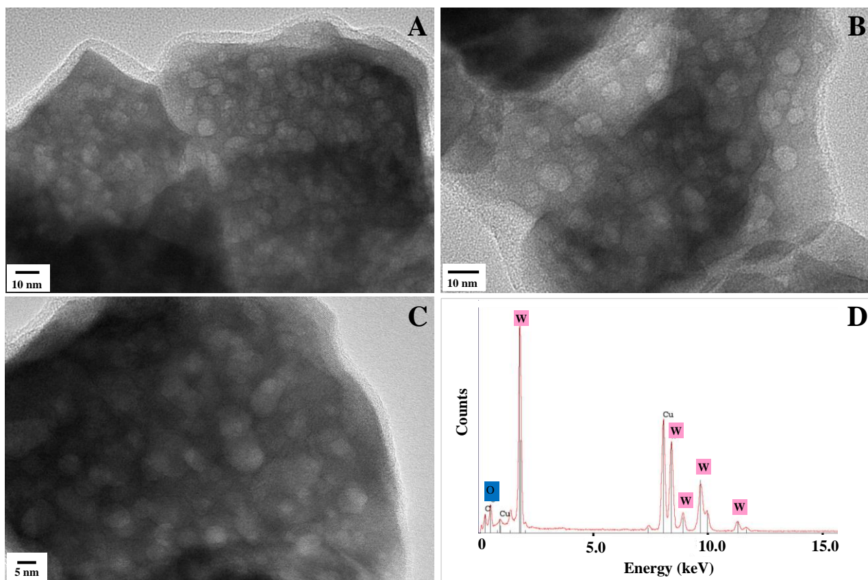
Fig. 3 HR-TEM images (A, B, C) and the EDX pattern (D) of mesoporous WO 3 thin films deposited by surfactant assisted electrodeposition (using SDS) at -0.5 V vs Ag/AgCl for 30 min, sample is thermally treated at 450°C for 2h.
