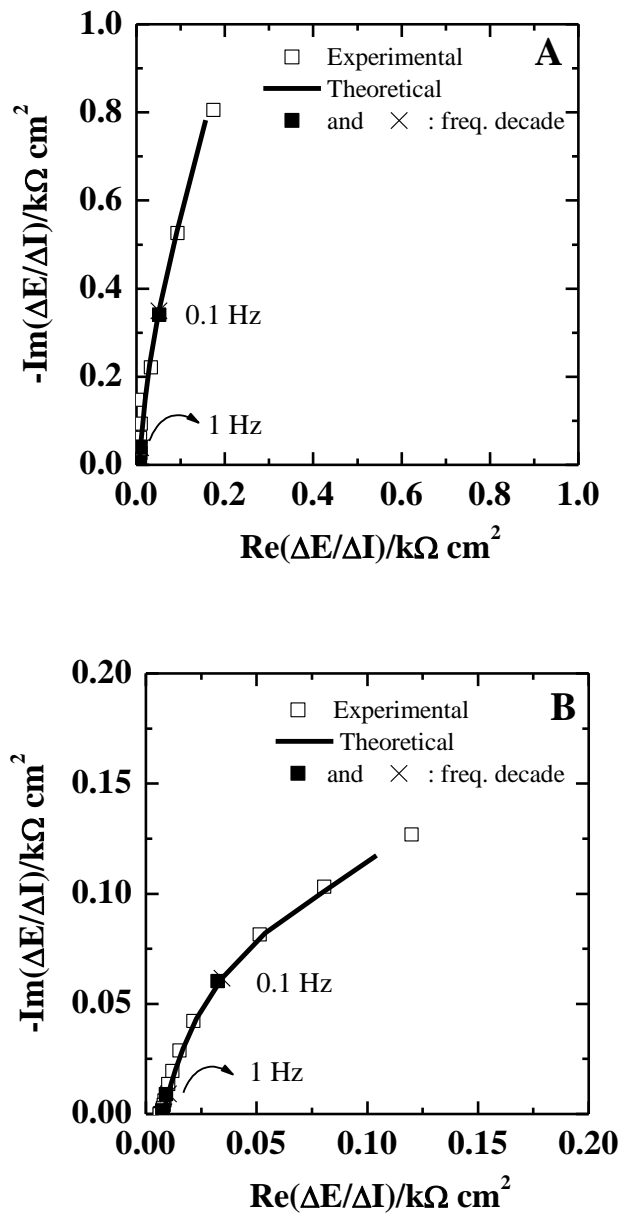
Fig. 7 The electrochemical impedance, \frac{\Delta E}{\Delta I}(\omega) for a dense (A) and a mesoporous (B) WO 3 thin film, measured in aqueous 0.5 M LiClO 4 electrolyte at -0.3 V vs Ag/AgCl (both experimental and theoretical curves are given).
