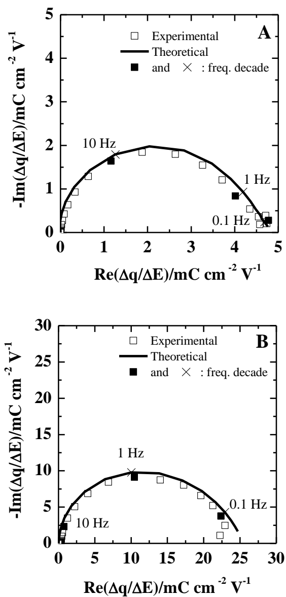
Fig. 8 Charge/potential transfer functions, \frac{\Delta q}{\Delta E}(\omega) for a dense (A) and mesoporous (B) \text{WO}_3 thin film measured in aqueous 0.5 M \text{LiClO}_4 electrolyte at -0.3 V vs Ag/AgCl (both experimental and theoretical curves are given).
