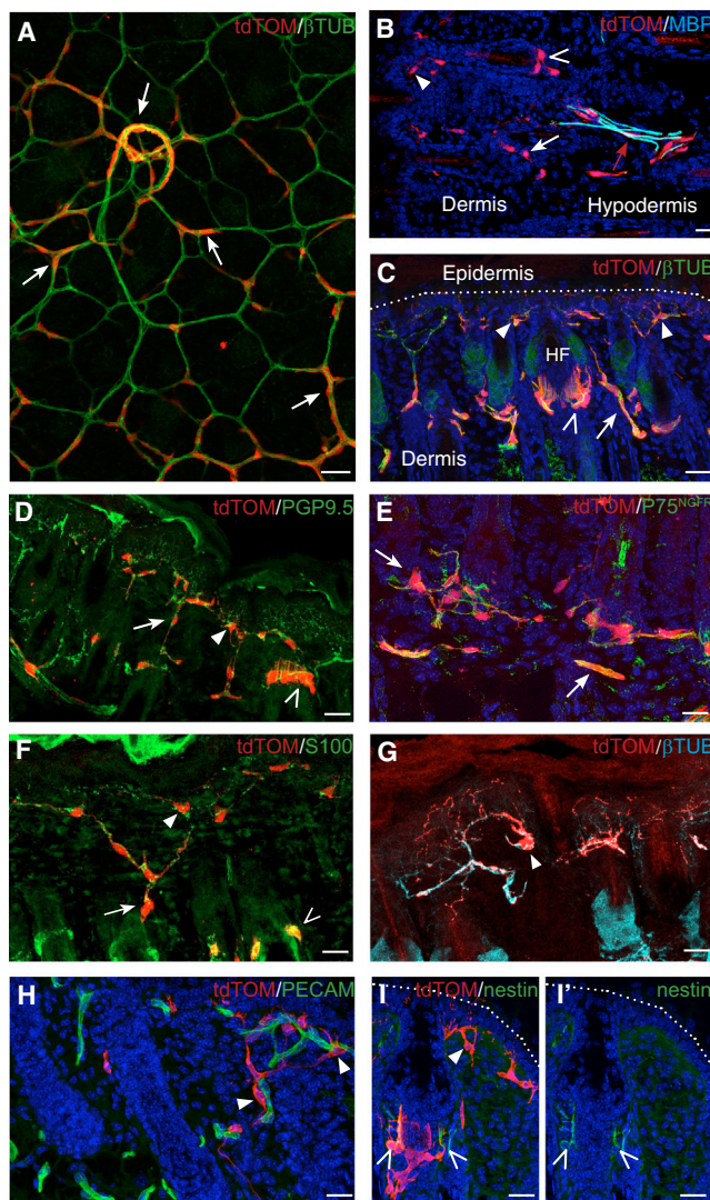
Figure 3. Identities of BC Derivatives in the Neonatal Skin (A) Whole-mount immunostaining of newborn skin from Prss56 Cre/+ , R26 tdTom animals for tdTOM and \beta III-tubulin, viewed from the hypodermal side. Most traced cells are in contact with the subcutaneous or dermal nerves (arrows). (B–I) Transverse sections of the skin from Prss56 Cre/+ , R26 tdTom newborn animals labeled with the indicated antibodies. In the hypodermis, traced cells are associated with the cutaneous nerves and some express the myelin marker MBP (B, red arrow). In the dermis, tdTOM-positive cells are localized along \beta III-tubulin-positive axons (C) and PGP9.5-positive terminal nerve fibers (D), and they express the NC stem cell/immature glial marker P75 NGFR (E) and the Schwann cell marker S100 (F), but not the myelin marker MBP (B, white arrow and open and closed arrowheads). These Schwann-like cells are associated with dermal nerves (A and C–F, arrows), free nerve endings (C, D, and F–I, closed arrowheads), or lanceolate endings of hair follicles (C, D, F, and I, open arrowheads). The cells associated with free nerve endings are highly ramified and are often in direct contact with blood vessels (G and H, arrowheads). Some of the traced
