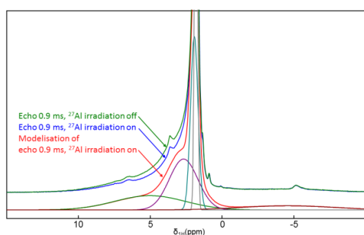
Figure 6. Echo MAS ^1\text{H} NMR spectra (sample dehydrated at 200^\circ\text{C} ). The chemical shift is based on \{^{27}\text{Al}\} - ^1\text{H} TRAPDOR experiment (spectra were simulated using dmfit program 26 ; see ESI)
