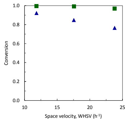
Figure 7. Conversion of ethanol at 400^\circ\text{C} with (■) SiAl(HIPE) and (▲) the reference. 1.2 g of catalyst. Selectivity to ethanol is always in the 94.2-97.6 % range (see Table S1 for full product profile). Feed is first generation bioethanol from BioWanze; 99.7wt.% ethanol – 0.3wt.% water evaporated in a preheating zone.
