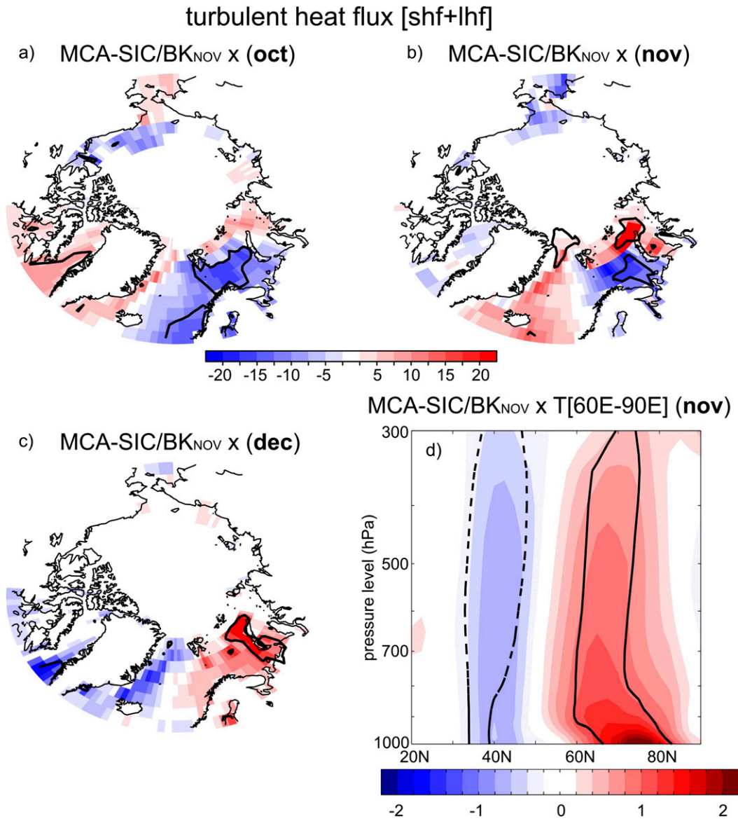
FIG. 8. Regression maps of detrended turbulent heat flux anomalies (sensible heat plus latent heat; W m^{-2} , upward is positive) in (a) October, (b) November, and (c) December onto the MCA-SIC/BK NOV expansion coefficient. (d) Regression cross section, pressure level vs latitude, of detrended air temperature anomalies zonally averaged over 60^{\circ} – 90^{\circ} E ( ^{\circ} C) in November onto the MCA-SIC/BK NOV expansion coefficient. Statistically significant areas at 95% confidence level based on a two-tailed Student's t test are contoured.
