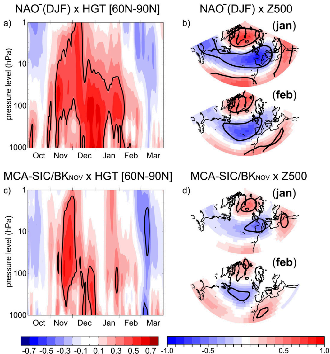
FIG. 10. (left) Correlation sections of detrended geopotential height anomalies averaged over the polar cap ( 60^{\circ} – 90^{\circ} N) with (a) the winter \text{NAO}^- index and (c) the \text{MCA-SIC/BK}_{\text{NOV}} expansion coefficient; the time axis is in daily values from 1 Oct to 31 Mar. (right) Correlation maps of detrended geopotential height anomalies at 500 hPa ( Z500 ) in January and February with (b) the winter \text{NAO}^- index and (d) the \text{MCA-SIC/BK}_{\text{NOV}} expansion coefficient. Statistically significant areas at 95% confidence level based on a two-tailed Student's t test are contoured.
