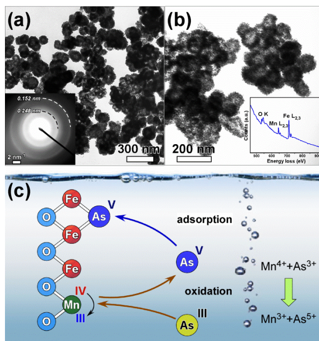
Fig. 2 Transmission electron microscopy images of hollow Fe oxyhydroxide (a) and Mn feroxyhyte nanostructures (b). Mechanism of Mn 4+ mediated adsorption of As(III) by Fe/Mn binary oxyhydroxides. 191,192
