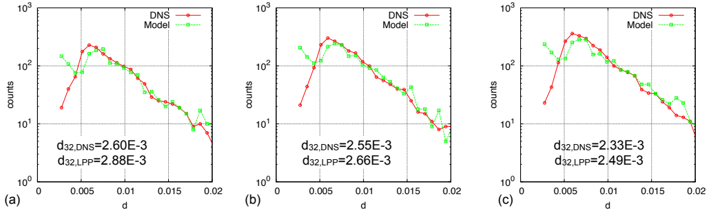
Figure 12: Size distribution and Sauter mean of droplets formed in pulsed-jet atomization at times (time units D_{jet}/U_{jet} ): (a) t = 8 , d_{32,DNS} = 2.60 mm, d_{32,LPP} = 2.88 mm , (b) t = 8.5 , d_{32,DNS} = 2.55 mm, d_{32,LPP} = 2.66 mm , (c) t = 9 , d_{32,DNS} = 2.33 mm, d_{32,LPP} = 2.49 mm .
