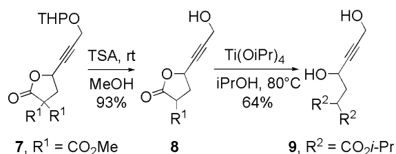
Scheme 4. Preparation of alkynyl diol 9 .
