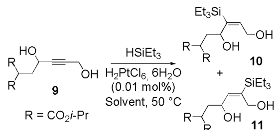
Figure 1. Hydrosilylation of 9 .
