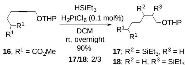
Scheme 6. Hydrosilylation of 16 .
