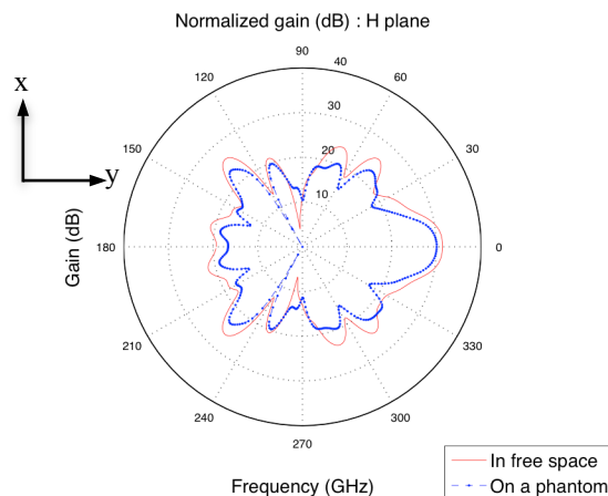
Fig. 6. Radiation pattern – phantom influence : H plane.
