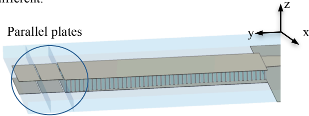
Fig. 1. SIW horn antenna design on CST : profile view.
