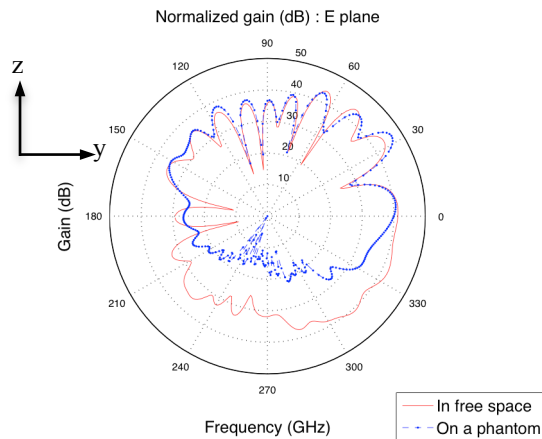
Fig. 7. Radiation pattern – phantom influence : E plane.
