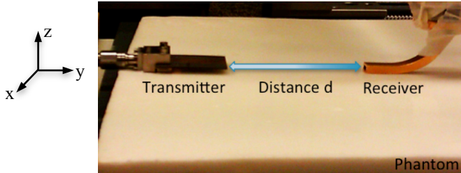
Fig. 8. Link characterization : SIW horn antenna to a waveguide.
