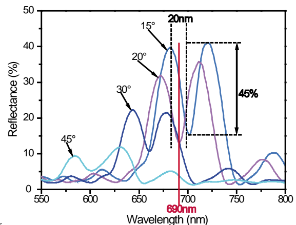
Figure 2. Specular reflection spectra of the heterostructure at different angles \theta .
