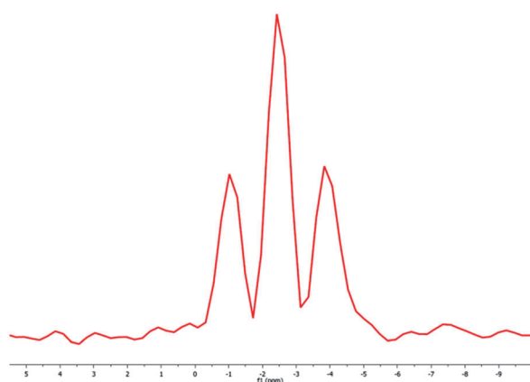
Fig. 7 Experimental 17 O spectrum of 20% enriched water, 55 mM in dioxane-d 8 , acquired on a 400 MHz NMR spectrometer. The binomial 1 : 2 : 1 distribution of the triplet due to J(^1\text{H}, ^{17}\text{O}) \sim 80 Hz is characteristic of an equilibrium Boltzmann distribution. Deviations from this binomial multiplet are expected if the TSI does not vanish, and could be a hallmark of para -water. Isotopic enrichment of 20% 17 O made it possible to use an acquisition time of a few seconds, making this method suitable for detection of a TSI.
