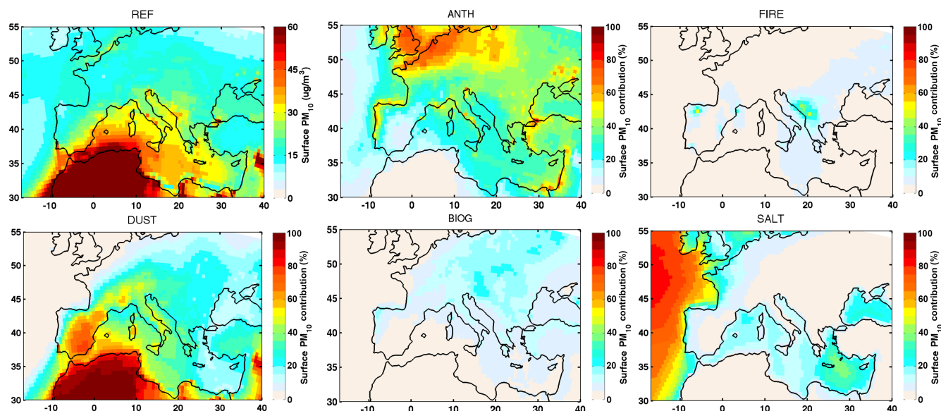
Figure 9. Relative contribution of each source type (i.e., the baseline simulation minus the sensitivity simulation where the respective source has been eliminated) to the simulated surface \text{PM}_{10} , averaged over the period (1 June to 31 August 2012). The top left represents the reference surface concentration over the same period.
