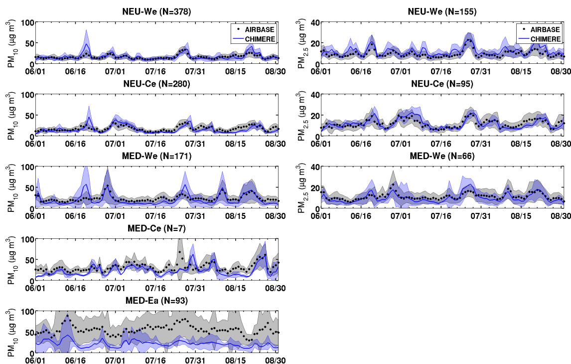
Figure 6. Temporal evolution during the summer of 2012 of observed daily mean surface PM 10 (left column) and surface PM 2.5 (right column) concentrations at AirBase and the two ChArMEs rural stations in Corsica (number in each region indicated by the value of N ), in addition to corresponding and collocated simulated daily mean surface concentration from CHIMERE (blue line). The corresponding standard deviation is indicated by a shaded area.
