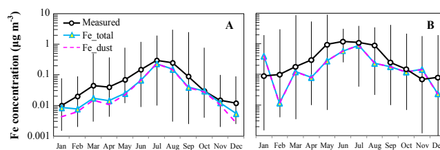
Figure 10. Seasonality of Fe concentrations attached to aerosols in surface air at Bermuda (32.2° N, 64.5° W) (a) and Barbados (13.2° N, 59.3° W) (b) on the western margin of the Atlantic Ocean. Modelled Fe concentrations are derived from all sources (Fe total ) and from mineral sources only (Fe dust ) as medians of all days of each month of 2005. Measured Fe concentrations are shown as the medians (circles) for 1988–1994 with the ranges between the 10th and 90th percentiles (error bars).
