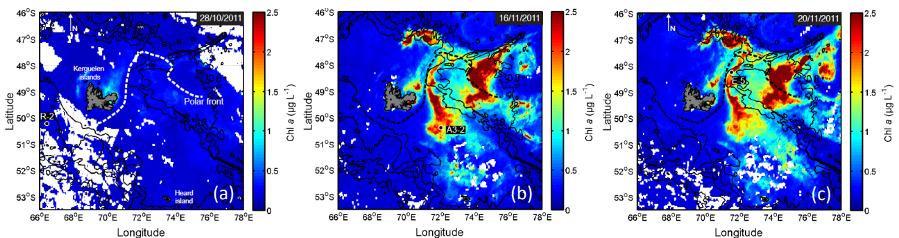
Figure 2. MODIS ocean-colour satellite images showing the development of the plateau and plume blooms during KEOPS-2. Surface chlorophyll ( \mu g L^{-1} ) biomass is shown for the nearest clear sky day to the final sampling day at stations R-2 (a), A3-2 (b) and E-5 (c). The PF is shown as a black dashed line in (b) and (c). Trull et al. (2015) discuss the timing of the stations relative to bloom development.
