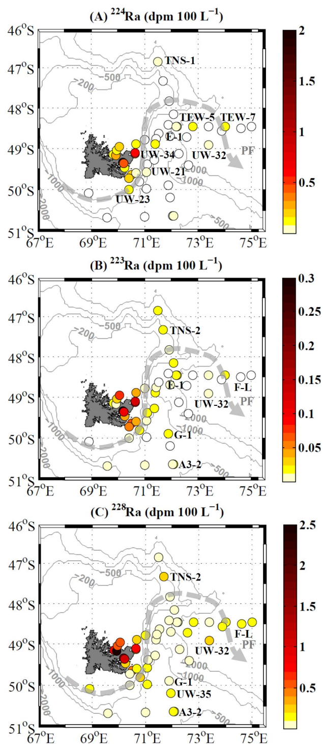
Figure 4. ^{224}\text{Ra} (a), ^{223}\text{Ra} (b) and ^{228}\text{Ra} (c) distributions in surface waters off the Kerguelen Islands. Radium activities are expressed in dpm 100 L ^{-1} . White circles indicate samples with Ra activity below the detection limit. A schematic view of the polar front (PF) is shown.
