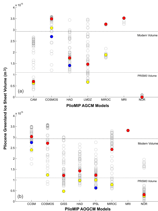
Figure 7. Simulated GrIS volume when BASISM is forced with the mPWP climatology from each of the (a) AGCM and (b) AOGCM PlioMIP models. The volume of the observed present-day GrIS (Bamber et al., 2001) is shown for comparison. Red-filled circles show the standard parameter set used within BASISM ( \alpha_i = 8 \text{ mm day}^{-1} \text{ }^{\circ}\text{C}^{-1} and \alpha_s = 3 \text{ mm day}^{-1} \text{ }^{\circ}\text{C}^{-1} , lapse rate = -6 \text{ }^{\circ}\text{C km}^{-1} ) and blue-filled circles show the parameter set that gives a volumetric reconstruction closest to observed. Yellow-filled circles show the parameter set that gives the smallest RMSE in terms of simulated ice sheet thickness. Grey circles show the sensitivity of the ice sheet volume to different values of lapse rate and the PDD factors for ice and snow (see Table 2). The coloured circles are superimposed on the grey circles, so when the GrIS volume is similar, the grey circles (or individual colours) will not be visible.
