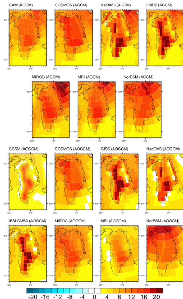
Figure 2. mPWP minus pre-industrial mean annual surface air temperature (°C) over Greenland for the PlioMIP ensemble using atmosphere-only (AGCMs) and coupled atmosphere–ocean climate models (AOGCMs). Temperature plotted on the original climate model resolution.
