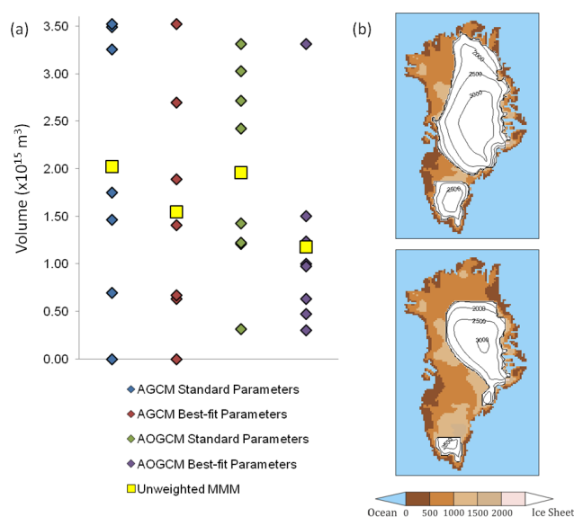
Figure 13. (a) Summary of the spread of mPWP GrIS volumes for each model within the PlioMIP ensemble (AGCM and AOGCM) compared with the un-weighted MMM for either the standard BASISM glaciological parameter set or for the parameter set that gives the “best” volumetric representation of the modern GrIS. (b) Ice sheet configuration with the closest volume equating to the largest (top) and smallest (bottom) MMM volume.
