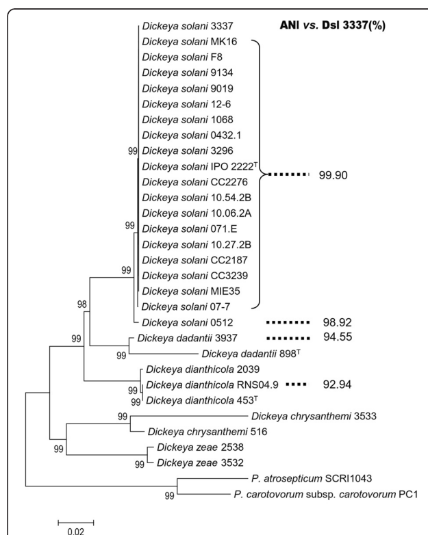
Fig. 1 MLSA and ANIs of D. solani strains. In MLSA the sequences of the genes ( rpoD , gyrB , recA , rpoS , dnaX , dnaA , gapA , fusA , rplB , purA , gyrA ) were aligned with ClustalW, and a Neighbour-joining tree was created by Bootstrap method with 1000 bootstrap replications. ANI values were calculated using Dsl 3337 as a reference
