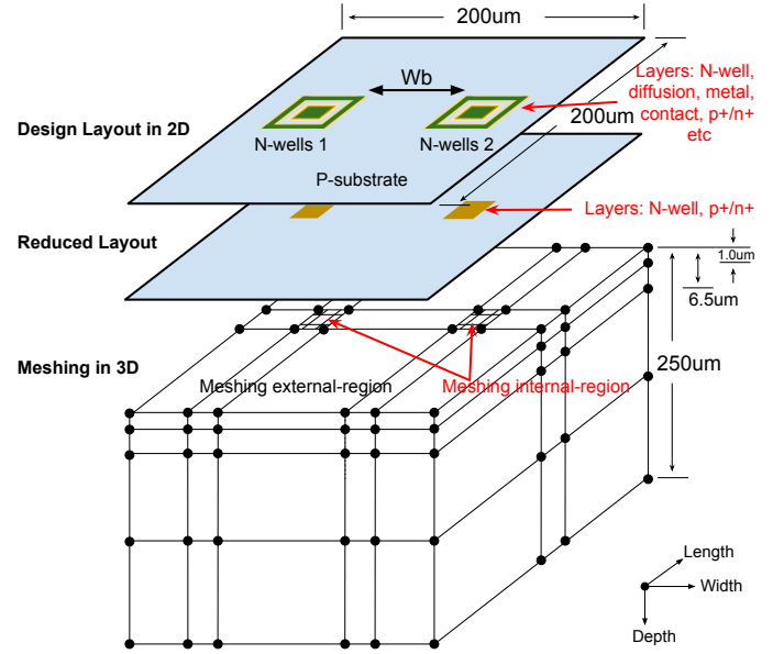
Fig. 3: Pre-processing of design layout.
