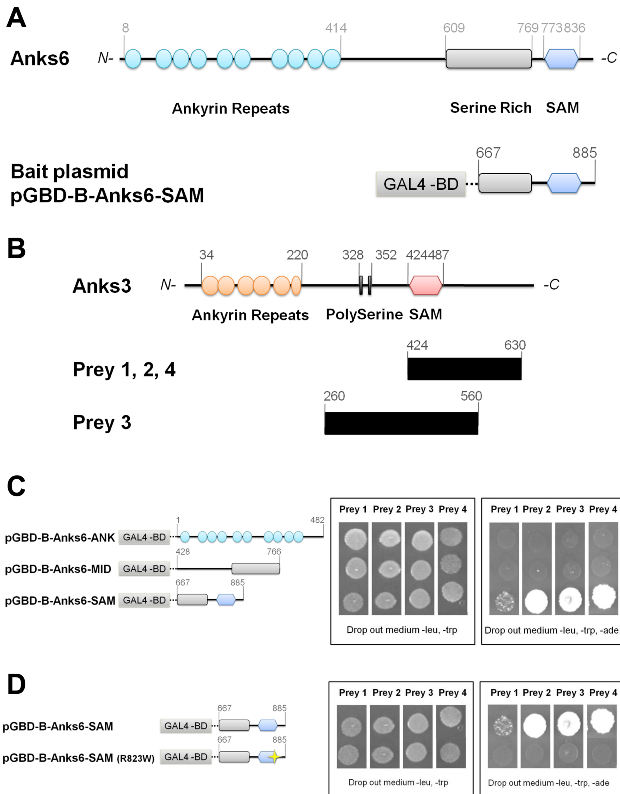
Fig 1. Identification of ANKS3, a partner of ANKS6. (A) Schematic representation of ANKS6 protein and the bait construct (pGBD-B-Anks6-SAM) used to perform the yeast two hybrid screen. (B) Schematic representation of ANKS3 protein for comparison with cDNA sequences of prey 1, 2, 3 and 4, recovered from the yeast two hybrid screen. (C) Interaction of ANKS6 with the 4 preys in interaction assays in yeast. The bait constructions containing either the Ankyrin
