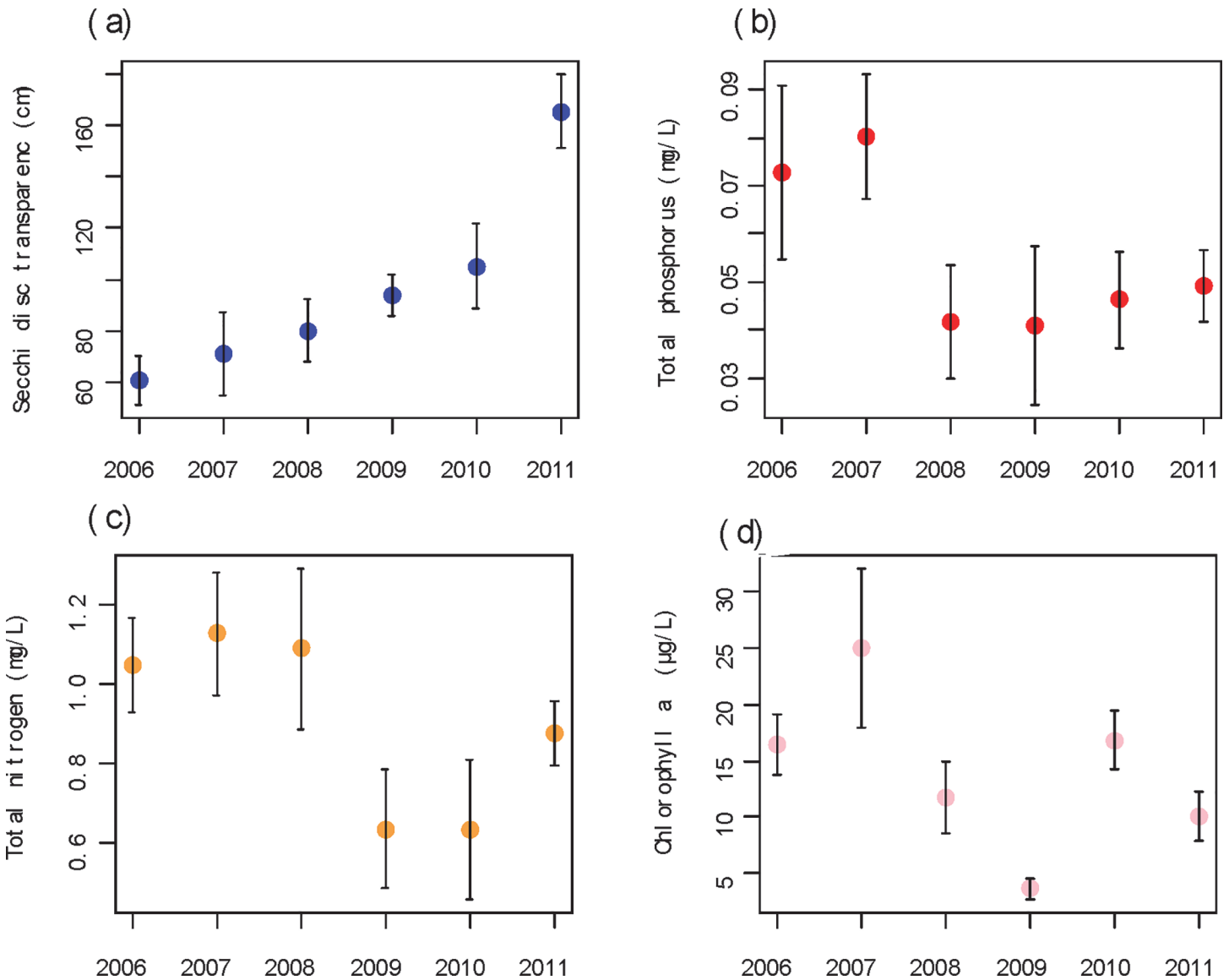
Fig 3. Water quality parameters of Wuhu Lake (China) before and after the start of bio-manipulation in 2008.
