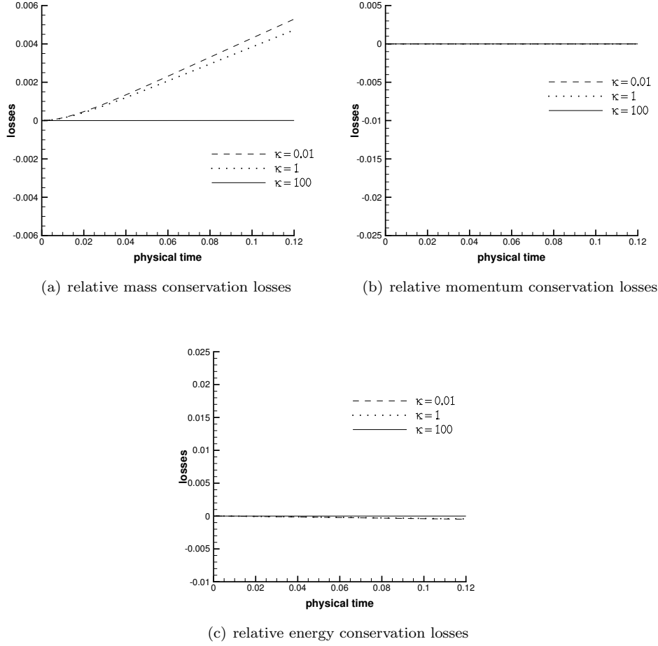
FIG. 4.10. Relative conservation losses for test case 5.
