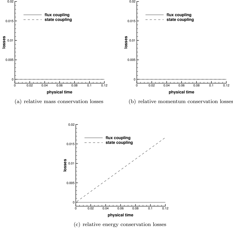
FIG. 4.2. Relative conservation losses for test case 1.
