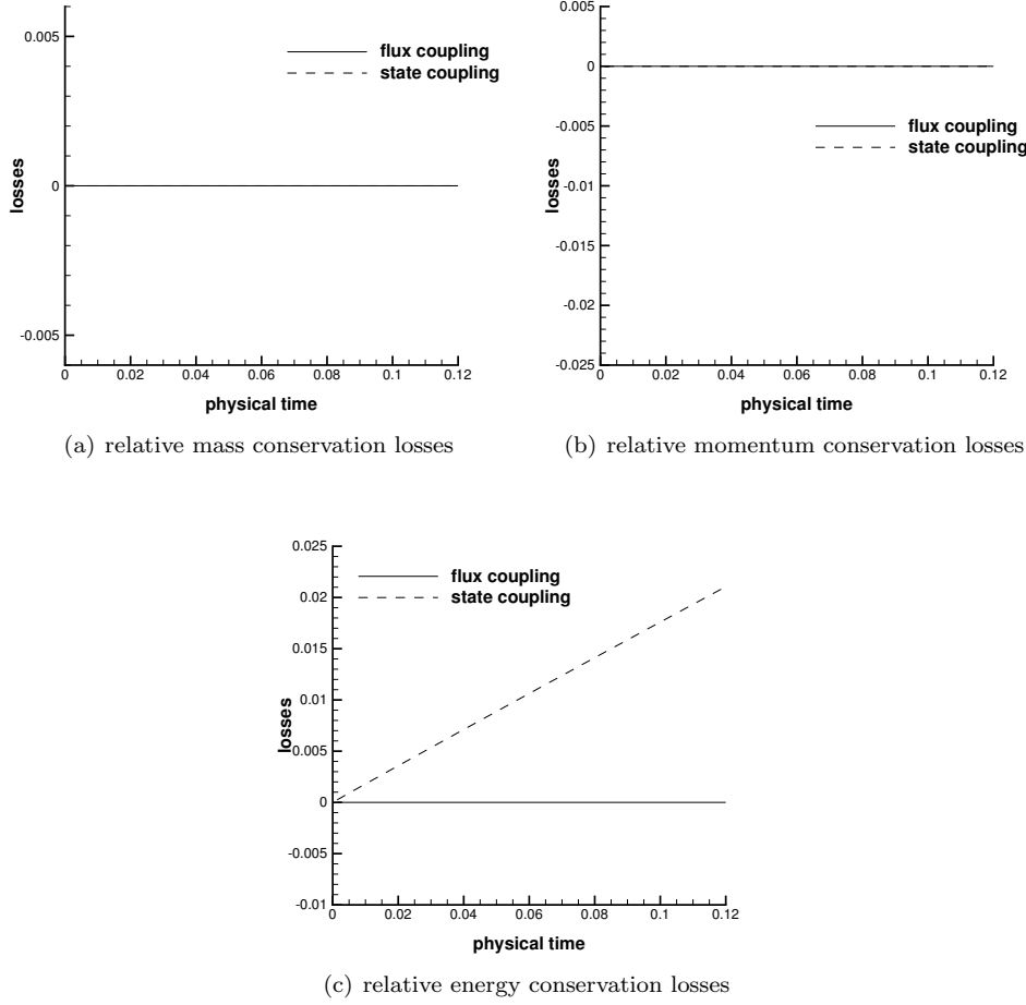
FIG. 4.4. Relative conservation losses for test case 2.
