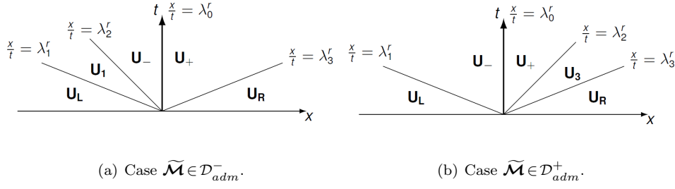
FIG. 3.2. The two possible wave structures of the solution of the Riemann problem (3.16).
