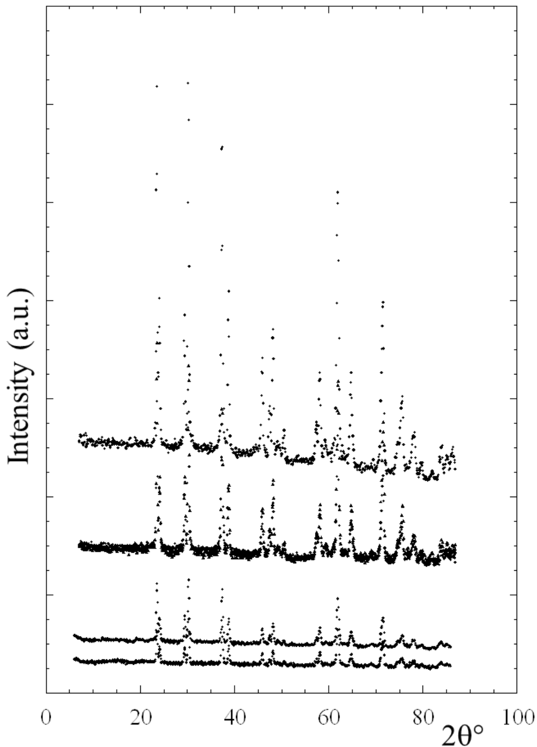
Fig. 5. Different Scattering diagrams collected on G4.1 on whewellite kidney stones.
