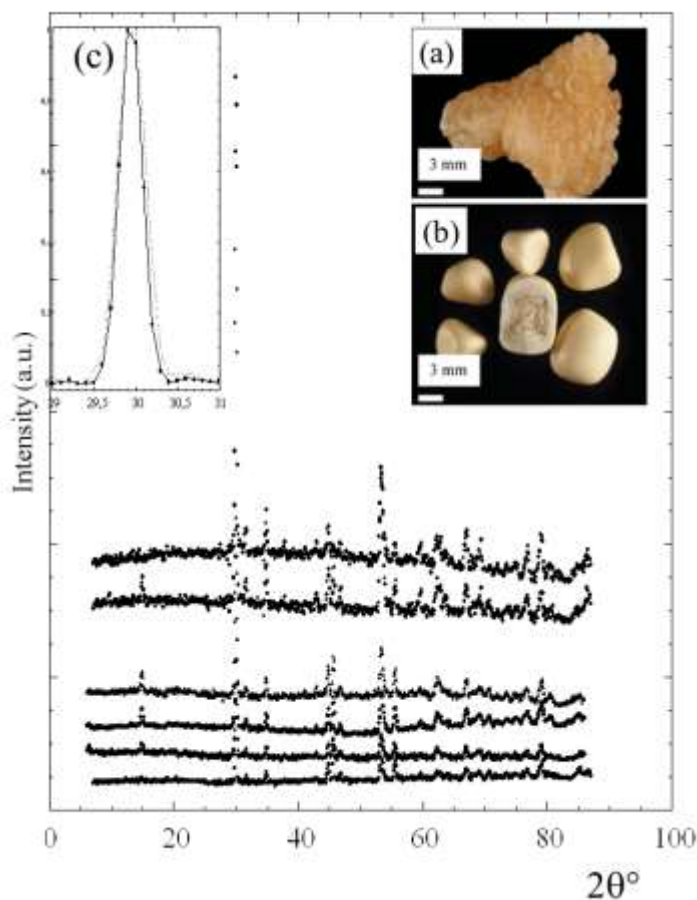
Fig. 4. (a) Va cystine kidney stone, (b) Vb cystine kidney stones. The cross section of a stone reveals a diffuse concentric structure at the periphery, and an unorganized agglomerate of cystine crystals in the core (c) typical neutron diffraction diagrams of cystine kidney stones collected on the G4.1 beamline (insert : illustration of the broadening of a Bragg peak, corresponding to the decrease of the crystallite size after treatment with sodium carbonate alkaline therapy).
