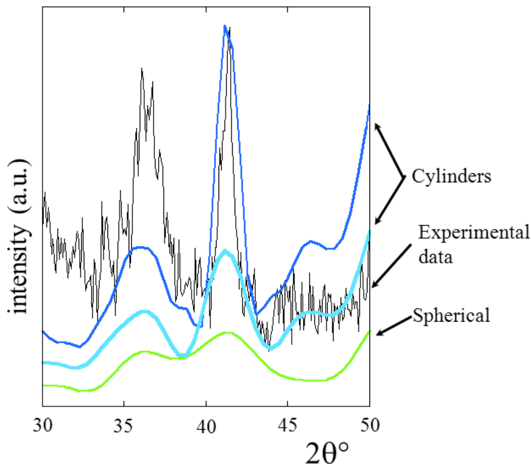
Fig. 6. Scattering diagrams calculated following the Debye formulae for different morphologies (cylinders and spherical) compared with experimental data.
