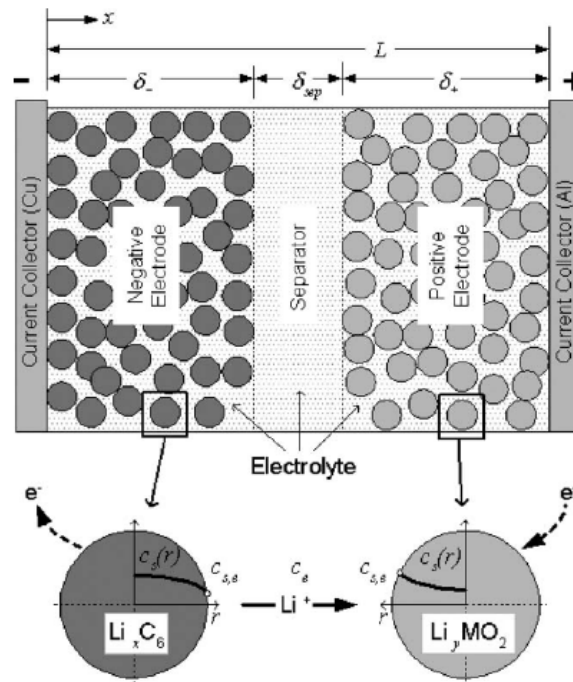
Figure 3: Diagram of 1D (x-direction) electrochemical cell model with coupled 1D microscopic (r-direction) solid diffusion model (reproduced from ref. [28]).
