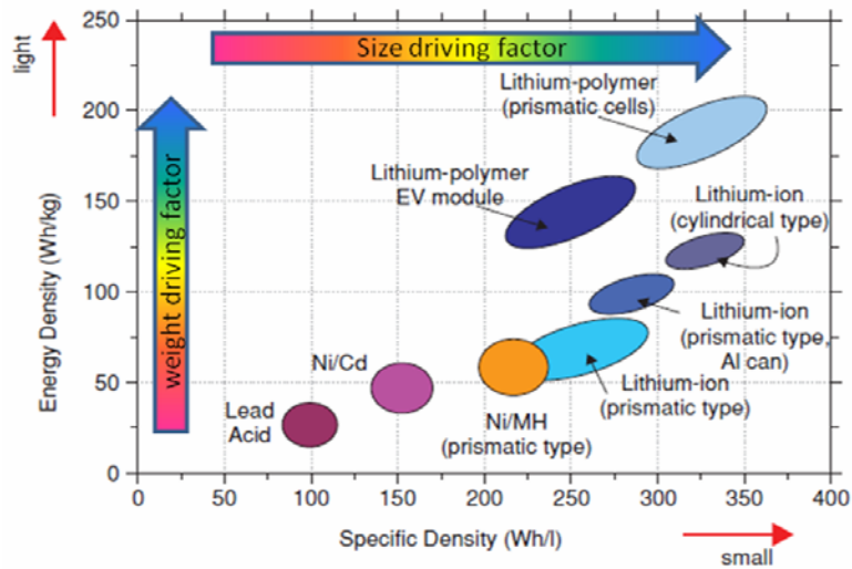
Figure 1: Energy density (Wh/kg) vs. specific density (Wh/L) diagram for a series of batteries (adapted from ref. [2])
