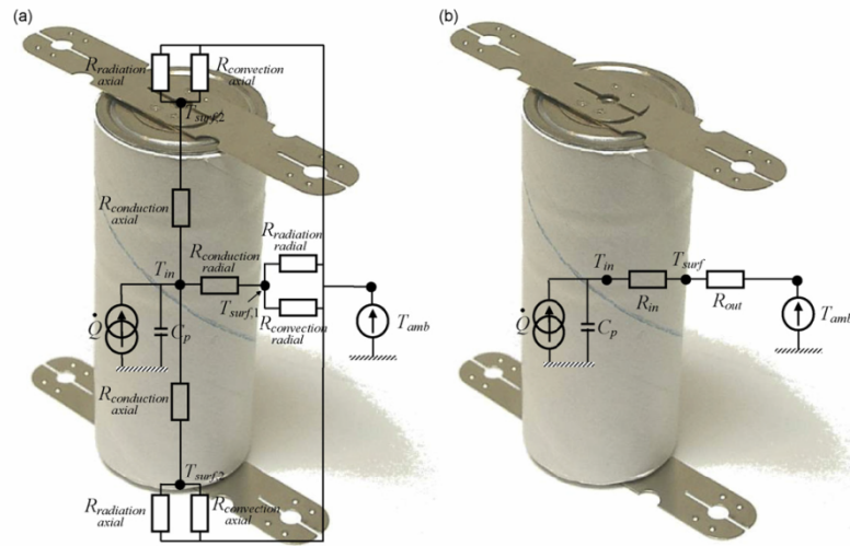
Figure 5: Forgez et al.'s Lumped models (a) complete model (b) simplified equivalent circuit model (adapted from ref. [76])
