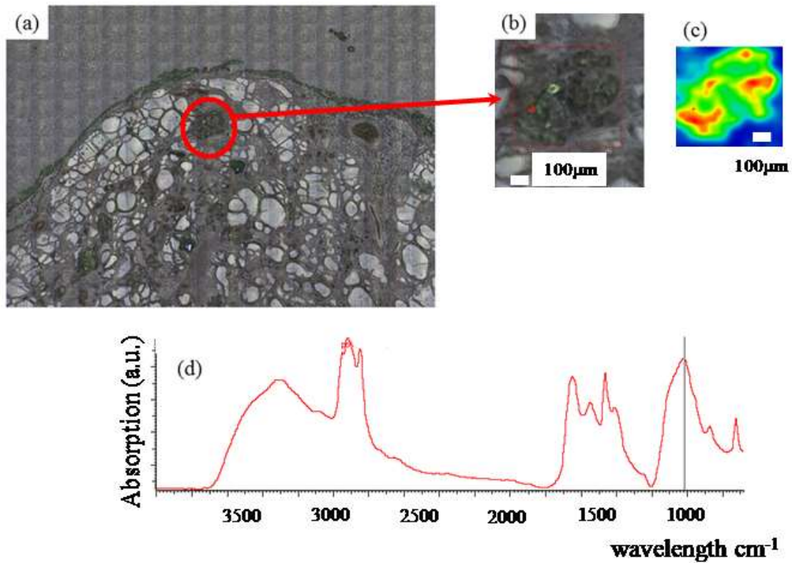
Fig. 4. Thyroid tissue (a) and (b) Optical photography at different scales, (c) Spatial distribution of phosphate apatite (d) FTIR spectra showing a absorption peak indicating the presence of apatite.
