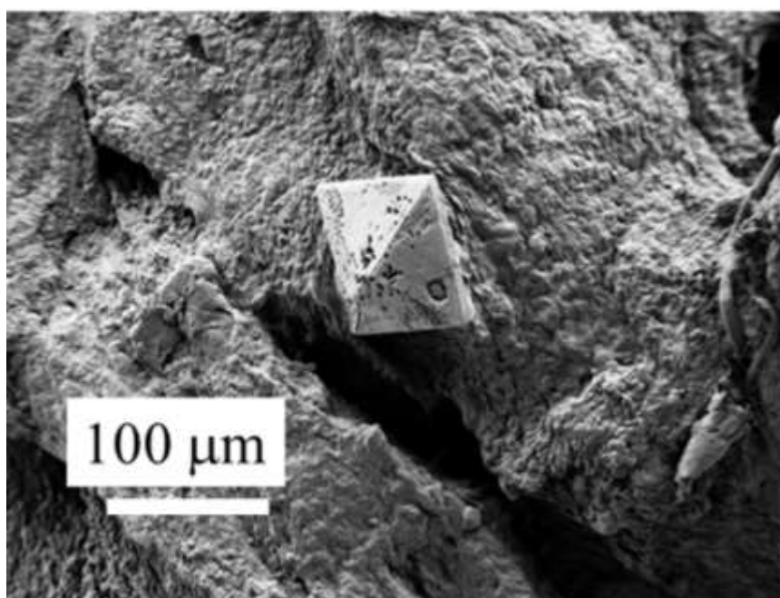
Fig. 3. SEM image of calcium oxalate dihydrate (weddellite) crystallite
