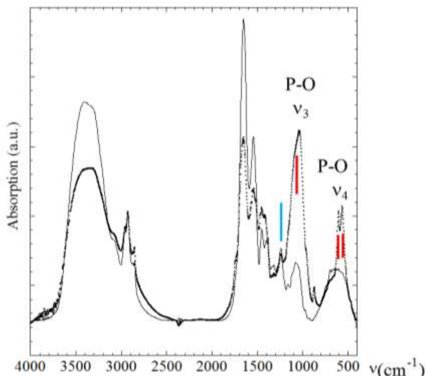
Fig. 1. FTIR absorption spectra collected for sample 5 (dots) and sample 6 (line). Red lines correspond to \nu_3 P-O stretching vibration modes measured at 1035\text{-}1045\text{ cm}^{-1} and O-P-O \nu_4 bending mode (doublet) at 602\text{-}563\text{ cm}^{-1} . Blue line corresponds to absorption peaks 1315 and 1318\text{ cm}^{-1} and at 780\text{ cm}^{-1} and is used to assess the presence of calcium oxalate in several samples, as weddellite [\text{CaC}_2\text{O}_4\cdot 2\text{H}_2\text{O}] and/or whewellite [\text{CaC}_2\text{O}_4\cdot \text{H}_2\text{O}] species.
