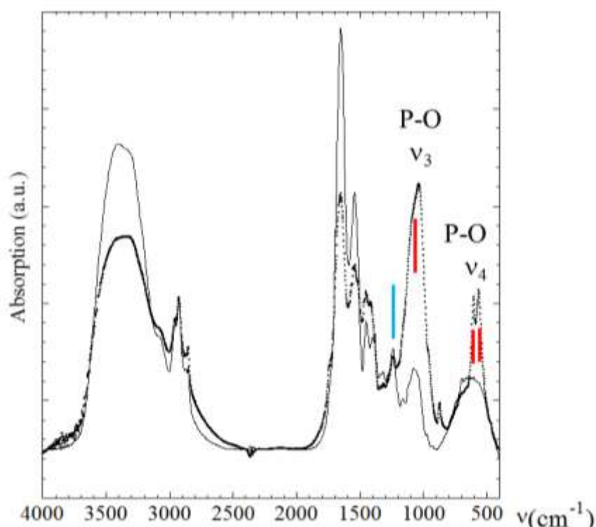
Fig. 1. FTIR absorption spectra collected for sample 5 (dots) and sample 6 (line). Red lines correspond to \nu_3 P-O stretching vibration modes measured at 1035\text{-}1045\text{ cm}^{-1} and O-P-O \nu_4 bending mode (doublet) at 602\text{-}563\text{ cm}^{-1} . Blue line corresponds to absorption peaks 1315 and 1318\text{ cm}^{-1} and at 780\text{ cm}^{-1} and is used to assess the presence of calcium oxalate in several samples, as weddellite [ \text{CaC}_2\text{O}_4\cdot 2\text{H}_2\text{O} ] and/or whewellite [ \text{CaC}_2\text{O}_4\cdot \text{H}_2\text{O} ] species.
