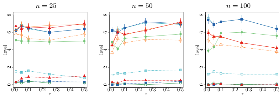
FIG 1. Estimated test levels in percentage under \mathcal{H}_0 for varying magnitudes of common non null coefficients, based upon 1000 simulations. Bonferroni calibration in dotted lines, calibration by permutation in plain lines. Blue squares represent the suggested test T_{\hat{\mathcal{S}}}^* , red triangles stand for the Fisher test T_{\hat{\mathcal{S}}}^{*,\text{Fisher}} . The deterministic collection \mathcal{S}_1 is drawn in empty points, while the data-driven collection \hat{\mathcal{S}}_{\text{Lasso}} is in plain points. Green circles represent the DiffRegr procedure, respectively plain and empty for single-splitting and multi-splitting.
