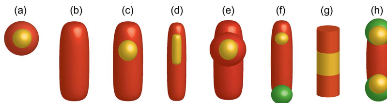
Fig. 1. Schematics of various colloidal structures. (a) Spherical core/shell nanocrystal, (b) nanorod, (c) core/shell dot-in-rod, (d) core/shell rod-in-rod, (e) bulb-shaped dot-in-rod, (f) CdSe/CdS–Pt dot-in-rod, (g) segmented nanorod heterostructure, and (h) double heterojunction nanorod.
