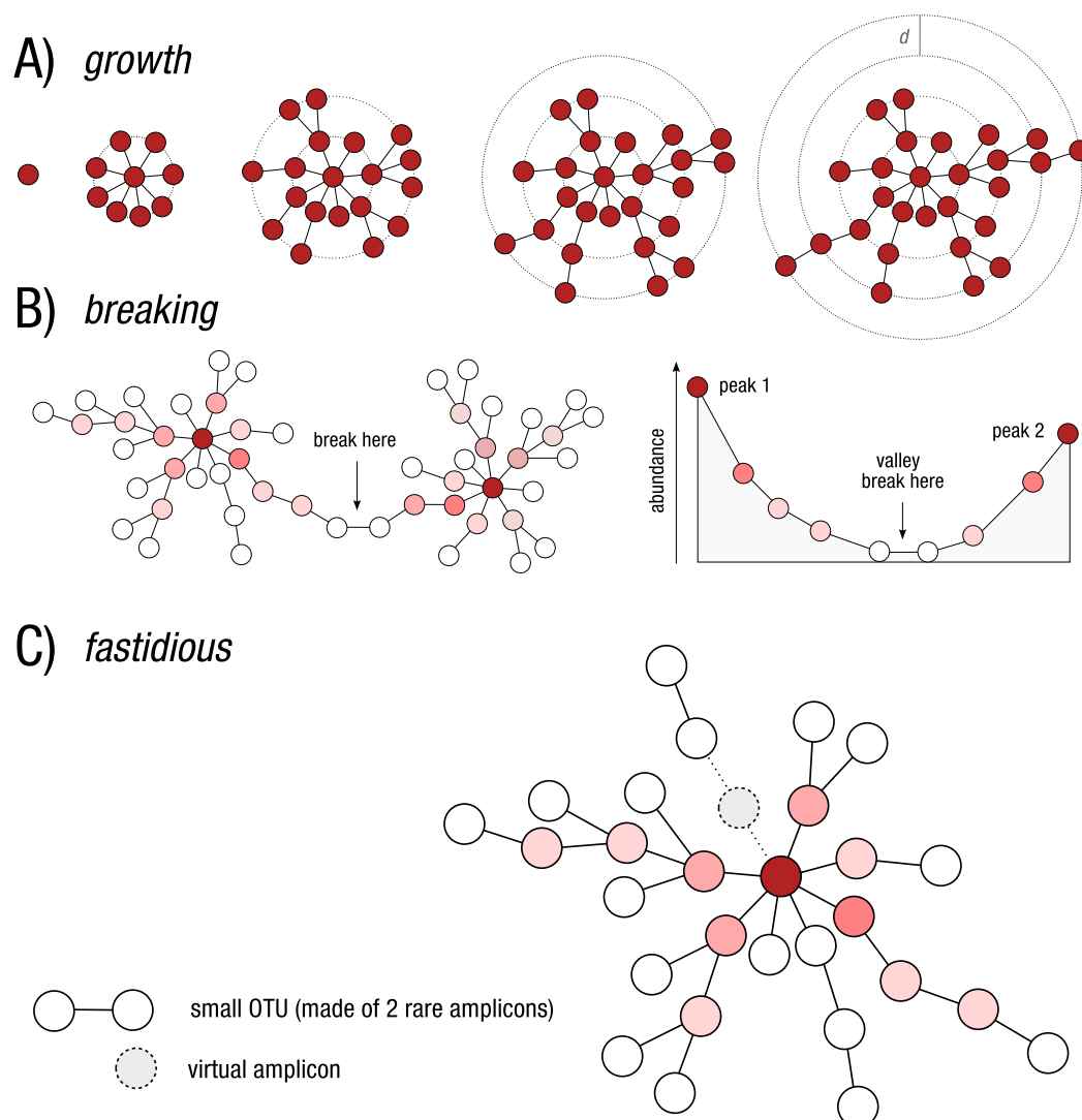
Figure 1 Schematic view of Swarm's clustering and refinement approach. (A) Swarm clusters amplicons iteratively by using a small user-chosen local threshold, d , allowing OTUs to grow to their natural limits, where no other amplicons can be added. (B) Swarm takes into account the abundance of each amplicon to produce higher resolution clusters, by not allowing the formation of amplicon chains. The darker the red, the higher the abundance. (C) The fastidious option avoids under-grouping (e.g., the production of small OTUs such as singletons and doubletons) by postulating the existence of virtual linking amplicons to graft smaller OTUs onto larger ones.
