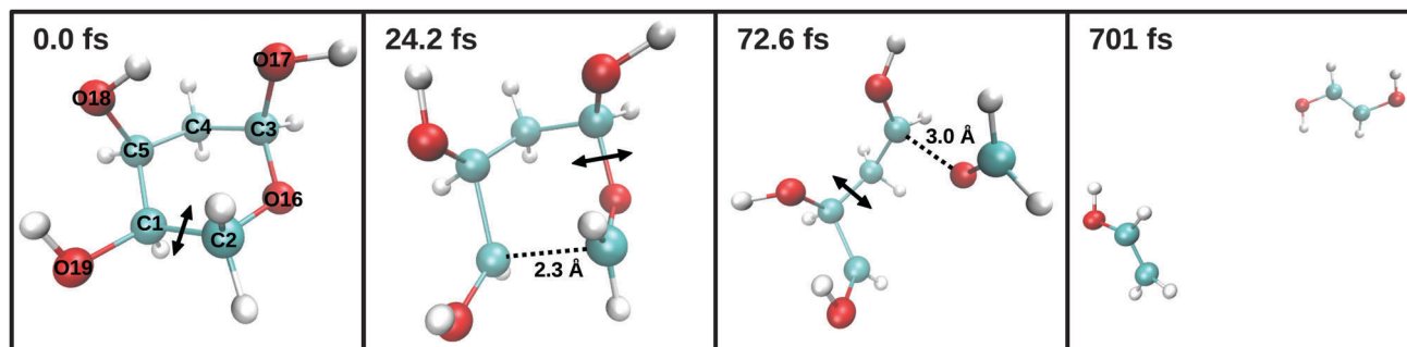
Fig. 3 BOMD trajectory initiated from an electronic configuration where two electrons were removed from the HOMO of the deoxyribose molecule (left, t = 0 ). The C_4O_3H_8^{2+} fragment was isolated during the last 290 fs of the dynamics. Bond breakage positions are marked by arrows. C blue, O red, H white.
