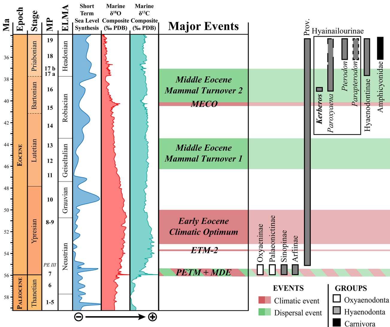
Fig 1. Stratigraphic repartition of the different subfamilies of specialized carnivorous mammals in Europe during the Paleocene and Eocene, with special attention to hyainailourines. The new taxon described here, Kerberos langebadrae , is in bold. Note that currently i. the stratigraphic extension of Paroxyaena pavlovi during Priabonian is unknown [8] and ii. the age of Parapterodon is unknown but is estimated to be late Priabonian [9]. Stratigraphic scale, eustatic curve, and isotopic curves produced with TSCreator [10] from the data compiled by Gradstein et al. [11]. Abbreviations: ELMA, European Land Mammal Ages; MP, Mammal Palaeogene.
