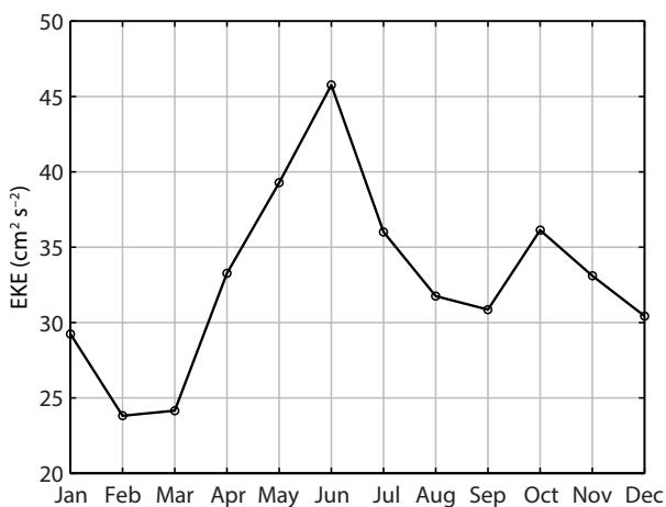
FIGURE 4. Geostrophic eddy kinetic energy (EKE) averaged over a 2^\circ \times 2^\circ box centered on the nominal location of the SPURS mooring (24.5°N, 38°W) as computed from the unbiasing method that combines satellite altimetry, drifter, and wind reanalysis data described by Centurioni et al. (2008). The EKE values were computed from the AVISO altimetry data set and averaged for each month of the year to compute the seasonal cycle.
