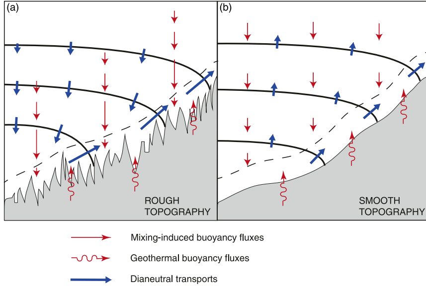
FIG. 3. Idealized schematic of local diapycnal transports induced by geothermal heat fluxes and internal wave breaking above (a) rough or (b) smooth bathymetry. In (a), the thin red arrows depict local downward buoyancy fluxes associated with bottom-intensified mixing parameterized by (19) and (20), accounting for their sharp decay in a relatively thin bottom layer (dashed line) of reduced mixing efficiency. The induced large-scale diapycnal transports (thick blue arrows) are directed toward higher (lower) density outside (within) the bottom layer. Thick black lines represent selected neutral surfaces. In (b), as a comparison example, buoyancy fluxes and diapycnal transports resulting from weaker internal wave activity and decreasing energy dissipation with depth are sketched. In this chosen situation, diapycnal upwelling occurs everywhere in the water column but preferentially along the seafloor. Note that we plot buoyancy fluxes as straight vertical arrows instead of diapycnal arrows so as to visualize the regions of divergent vs convergent buoyancy flux and to be consistent with the present methods where local density fluxes are approximated as vertical.
