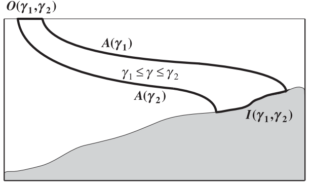
FIG. 1. Sketch of a neutral density layer \gamma_1 \leq \gamma \leq \gamma_2 bounded by neutral surfaces A(\gamma_1) and A(\gamma_2) and by its outcrop and incrop surfaces O(\gamma_1, \gamma_2) and I(\gamma_1, \gamma_2) .
