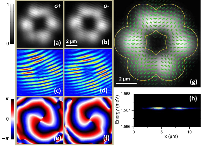
FIG. 5. Condensation in the k = 3 state of the E(2) manifold. (a,b) Real space emission in the \sigma_+ and \sigma_- circular polarizations for a polariton condensate in the state |\psi_{\text{lower}}(k = 3)\rangle , at 25 mW. Each polarization component contains a vortical current of double phase charge in the counterclockwise ( \sigma_+ ) and clockwise ( \sigma_- ) directions, evidenced in the double forklike dislocations apparent in the interferometric measurements shown in (c) and (d), respectively, and in the extracted phase gradients in (e) and (f). The phase changes from 0 to \pm 4\pi when circumventing the molecule. (g) The green traces show the plane of linear polarization of the emission measured locally, superimposed to the total emitted intensity of the molecule. At the center of each micropillar, the condensate shows a linear polarization pattern pointing radially. Solid lines depict the contour of the microstructure. (h) Spatially resolved emission spectrum.
