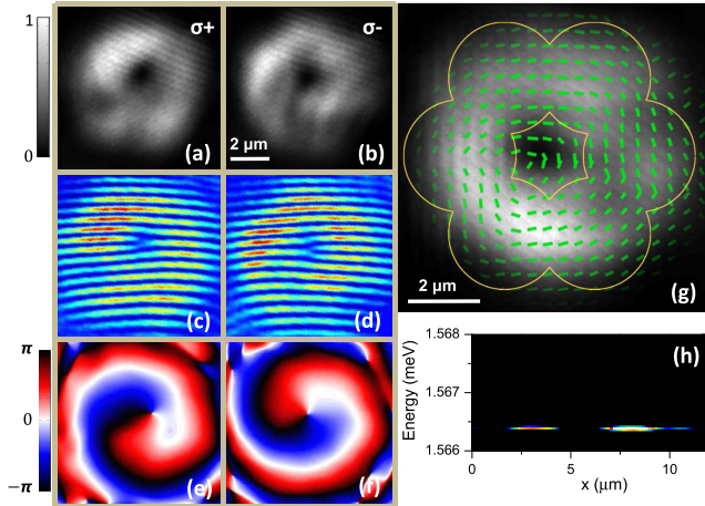
FIG. 4. Condensation in the k = 0 state of the E(1) manifold. (a,b) Real space emission in the \sigma_+ and \sigma_- circular polarizations for a polariton condensate in the state |\psi_{\text{lower}}(k = 0)\rangle , at a pumping intensity of 84 mW. Each polarization component contains a vortical current in the clockwise ( \sigma_+ ) and counterclockwise ( \sigma_- ) directions, evidenced in the forklike dislocations apparent in the interferometric measurements shown in (c) and (d), respectively, and in the extracted phase gradients in (e) and (f). The phase changes from 0 to \mp 2\pi when circumventing the molecule. (g) The green traces show the plane of linear polarization of the emission measured locally, superimposed to the total emitted intensity of the molecule. The condensate shows azimuthal linear polarization. Solid lines depict the contour of the microstructure. (h) Spatially resolved emission spectrum.
