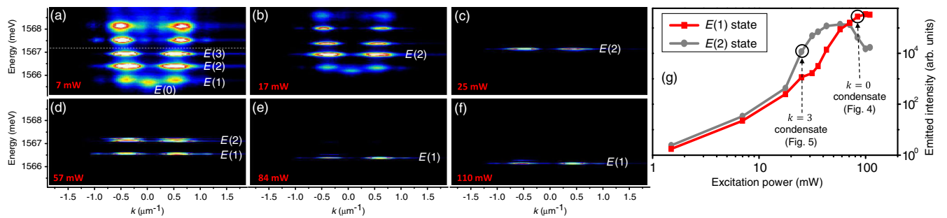
FIG. 3. Power dependence of the condensation process. (a)–(f) Energy- and momentum-resolved emission of the molecule as a function of the excitation power, indicated in each panel. At low power (a), the E(0) , ..., E(3) energy levels are visible along with higher energy states (above the dashed line) arising from the coupling of higher energy modes of each individual pillar [32]. When increasing the excitation power, polariton condensation occurs first in one of the states of the multiplet E(2) (c) and then in one of the states of the multiplet E(1) (e,f). In (d), the double line in E(2) arises from fluctuations in the position of the pump spot during the measurement (see Sec. E of Ref. [32]). These fluctuations were absent in the experiments shown in Figs. 4 and 5. (g) Emitted intensity of the E(1) and E(2) states as a function of the excitation power. The circles indicate the power at which the experiments shown in Figs. 4 and 5 were performed.
