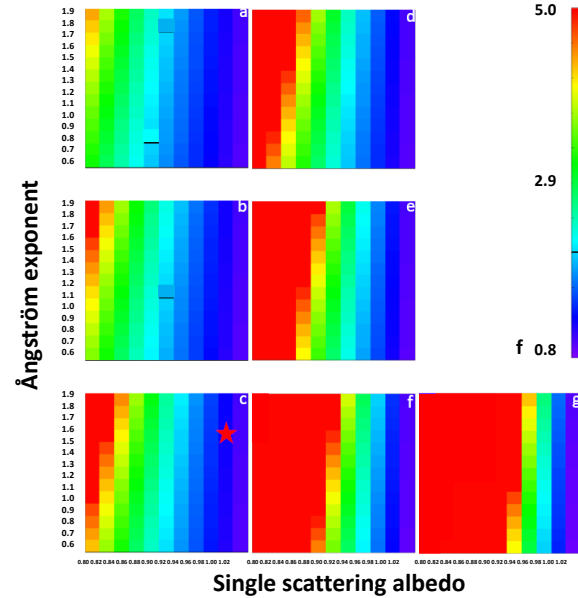
Figure 2: F ratio as a function of single scattering albedo SSA and Angstrom coefficient \alpha , for asymmetry factor g varying between 0.6 (a) to 0.9 (g). The red star indicates the SSA, \alpha and g values for the case study discussed in [Sellitto et al., 2015].
