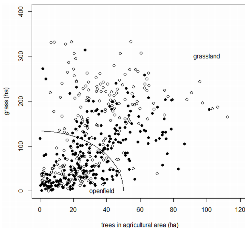
Figure 1 Stratification of the squares. “Openfield” and “grassland” on both sides of the curve defined by the Eq. (1) given in the text; closed circles: Southern temperate Atlantic ecoregion (“West”); open circles: Western European broadleaf forest ecoregion (“East”).
