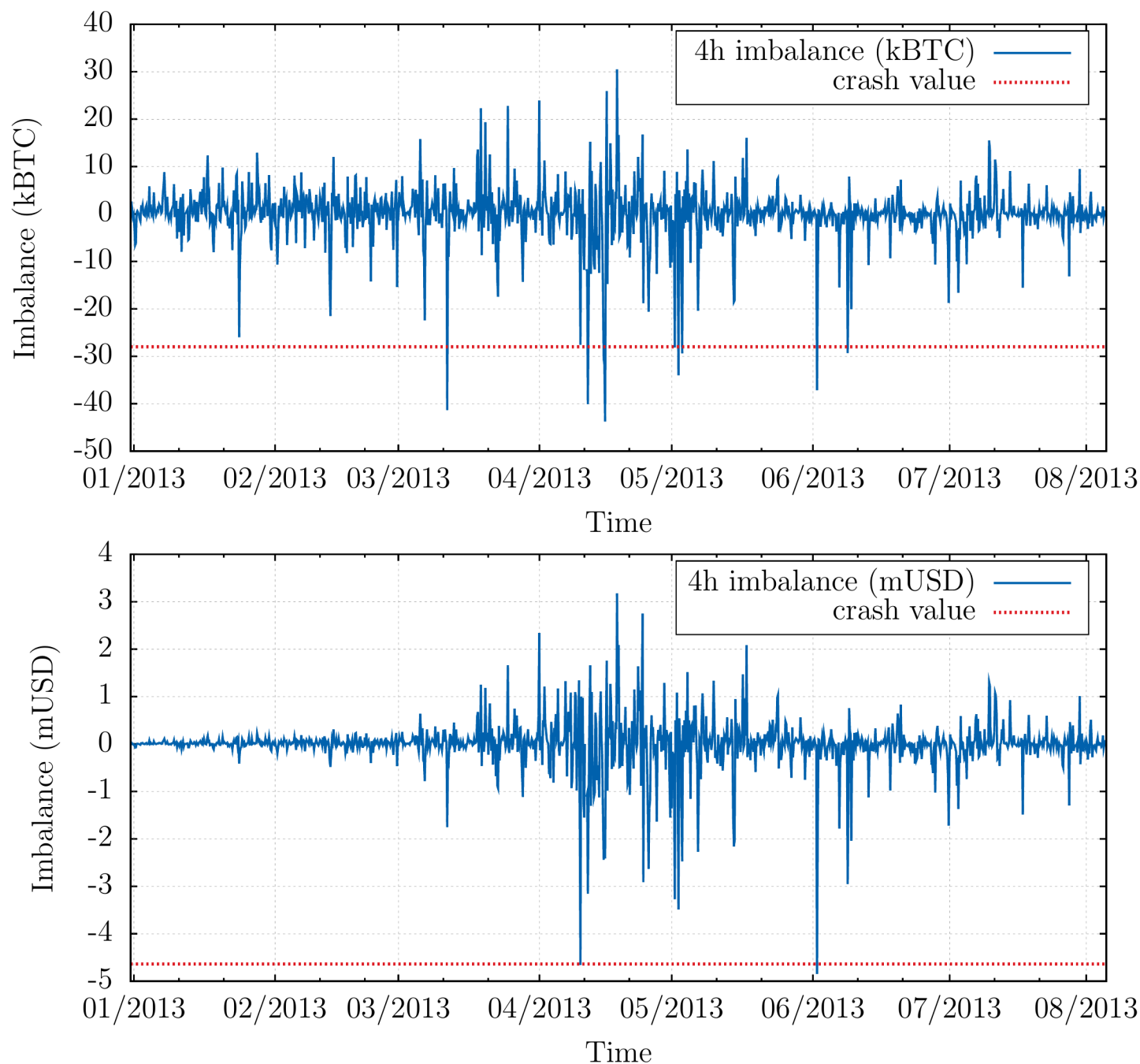
Fig 2. Order flow imbalances in USD and BTC. Top: Aggressive imbalance in order flow \sum_j \epsilon_j v_j (where \epsilon_j = \pm 1 is the sign of the transaction, and v_j its volume in Bitcoins), aggregated over periods of 4 hours between January 2013 and August 2013, expressed in Bitcoins. April 10, 2013 (for which the realised imbalance is represented as a dashed horizontal line) does not appear as an outlier. Bottom: aggressive imbalance in order flow \sum_j \epsilon_j v_j p_j , aggregated over periods of 4 hours between January 2013 and August 2013 and expressed in USD. April 10, 2013 now clearly appears as an outlier.
