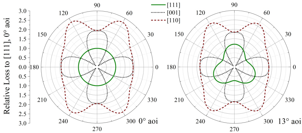
Fig. 7. Calculated angular depolarization loss maps for an \text{Yb}^{3+}:\text{YAG} crystal carrying three type of orientations. The left map is obtained for a double pass (active mirror architecture) extraction beam propagating through the disk at normal incidence (AOI 0^\circ ) whereas a 13^\circ AOI (corresponding to Lucia experimental case) is depicted on the right map.
