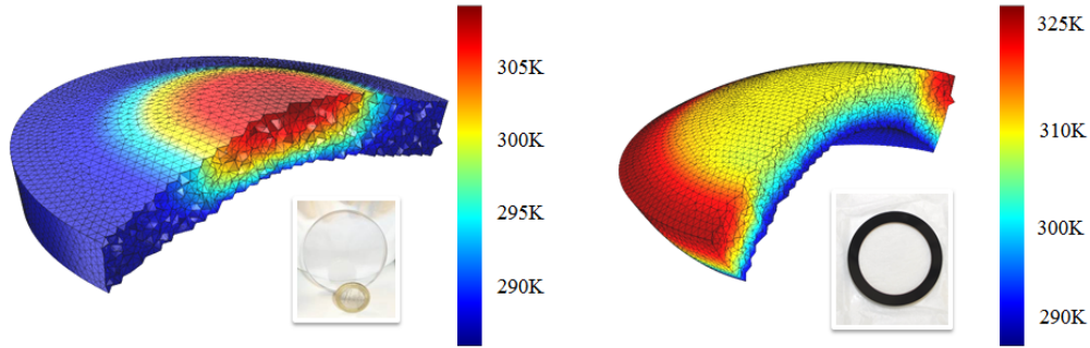
Fig. 5. 3D thermo-mechanical model of both crystal (left) and co-sintered ceramic (right) 7 mm thick YAG disks. 15 kW/m 2 /K heat exchanged coefficient water cooling takes place from the bottom (observe the cold blue surface) while pumping occurs on the top surface. The color temperature distribution clearly reveals the opposite radial temperature gradient of both cases. The heat source corresponds to a 16 kW/cm 2 pumping at 2 Hz, 1 ms.
