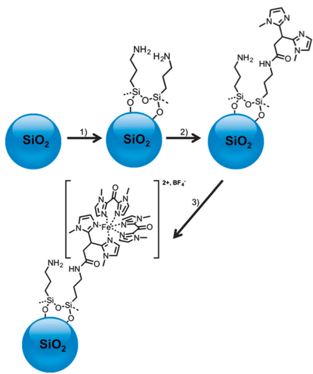
Scheme 1 Representation of the molecular architectures grafted at the surface of silica nanoparticles. (1) 3-Aminopropyltriethoxysilane, EtOH (2) HBIP, EDC, MeCN (3) [\text{Fe}(\text{BIK})_2(\text{MeCN})_2](\text{BF}_4)_2 .
