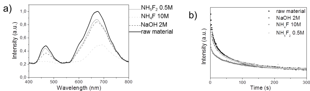
Figure 7. (a) Persistent luminescence spectra of C 0.3 M 1.7 S 3 O 9 : Eu1% Mn5% Dy2% depending on post-annealing treatment: NaOH 2M, NH 4 F 10M and NH 5 F 2 0.5M and (b) luminescence decay curves ( \lambda_{exc} = 365 \text{ nm} - t_{exc} = 120\text{s} ).
