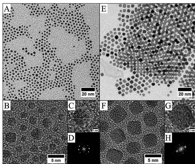
Fig. 2 Pt-C_8NH_2 nanoparticles synthesized under overpressure of H_2 from procedure I: TEM image (A) and HRTEM images (B–C) with FFT associated (D) and from procedure II: TEM image (E) and HRTEM image (F–G) with FFT associated (H).
