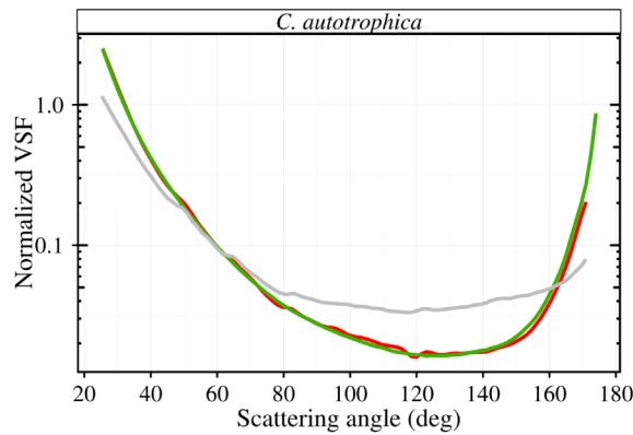
Fig. 5. Normalized volume scattering functions (VSF, in \text{sr}^{-1} ) of the species C. Autotrophica measured by the I-VSF (in red) and POLVSM (in green) instruments. The normalized VSF was calculated by dividing the VSF by the integrated value over the angular distribution available for each instrument. Filtrate measurements of VSF (blanks) are also shown (grey lines) for this species.
