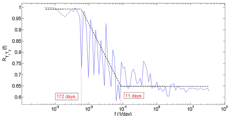
Fig. 5. Co-spectra in semi-log ( x axis) plot, of the temperature series in Roscoff and Boulogne-sur-Mer. There is a good correlation for scales larger than 172 days, a transition between 172 and 11 days, and a relative decorrelation for scales smaller than 11 days.
