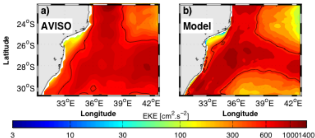
Figure 5: Mean eddy kinetic energy for (a) AVISO and (b) ROMS-SWIM (black contours indicate 600\text{ cm}^2\text{ s}^{-2} isolines).
