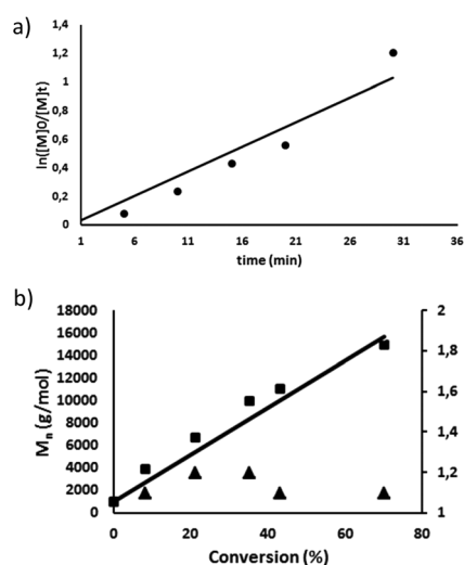
Fig. 2 (a) First-order kinetic plot for the RAFT polymerisation of DMAC using MePilla-CTA ; (b) dependence of the number-average molar mass ( M_n ) and dispersity ( D ) on conversion, for the RAFT polymerisation of DMAC in DMF using MePilla-CTA .
