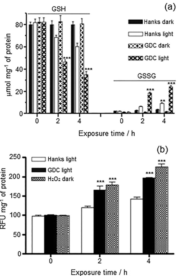
Figure 4. Effect of photosensitized reactions mediated by GDC on the redox status of bovine lens epithelial cells (BLEC). (a) Effect of ultraviolet A (UVA) visible irradiation in the presence of GDC on cytosolic levels of reduced glutathione (GSH) and oxidized glutathione (GSSG). Results are expressed as means \pm standard deviations ( n = 3 ), **p < 0.01 , ***p < 0.0001 compared to their respective controls (Hanks dark); (b) reactive oxygen species in BLEC after UV exposure in presence of GDC. The intensity of fluorescence caused by intracellular 2,7-dichlorofluorescein increased with UV exposure in a dose-dependent manner with time exposure. The measurement of reactive oxygen species (ROS) in the untreated cells was taken as 100%. As positive control, cells were incubated in the presence of \text{H}_2\text{O}_2 100 \mu\text{mol L}^{-1} for the same period of the experiment. Results are expressed as means \pm standard deviations ( n = 3 ), ***p < 0.0001 compared to their respective controls (time 0).
