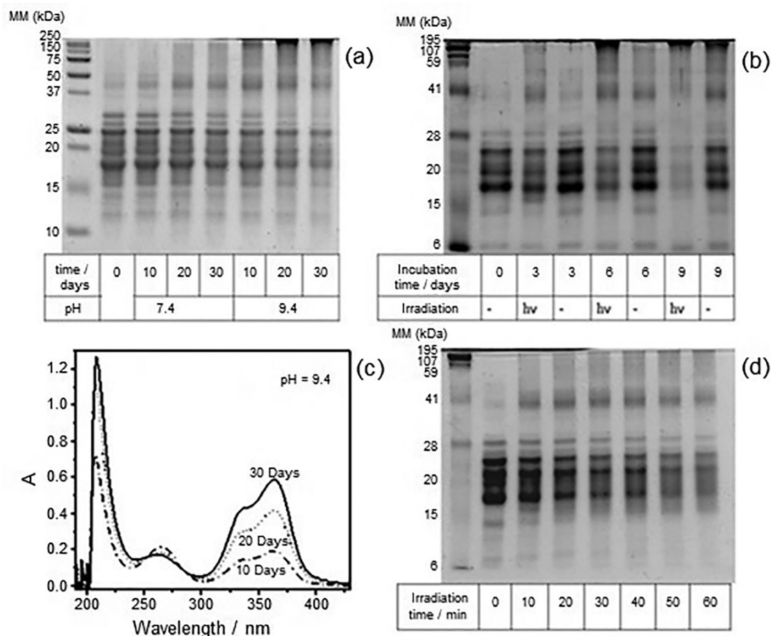
Figure 1. Eye lens proteins incubated with glucose, induce protein crosslinking in a pH-dependent manner and through ultraviolet A (UVA) visible light-induced photosensitized reactions mediated by a side product of the glucose degradation. (a) SDS-PAGE analysis of bovine lens proteins (10 mg mL -1 ) incubated with glucose 30 mmol L -1 for 10, 20 and 30 days at pH 7.4 or 9.4; (b) SDS-PAGE analysis for lens proteins (10 mg mL -1 ) incubated with glucose in the absence and presence of UVA-visible light; (c) absorption spectra of glucose (30 mmol L -1 ) incubated for 10, 20 and 30 days in sterile conditions at 37 °C, pH 9.4; (d) SDS-PAGE analysis of lens proteins (20 mg mL -1 ) irradiated with UVA-Visible light (at 5% O 2 ) and the presence of purified glucose degradation chromophore.
