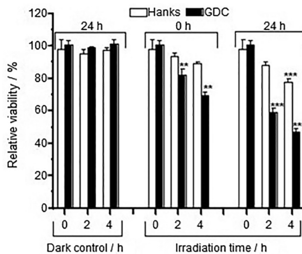
Figure 3. Effect of photosensitized reactions mediated by glucose derived chromophore on the viability of bovine lens epithelial cells. The cell viability was determined by means of the reduction of 3-(4,5-dimethylthiazol-2-yl)-2,5-diphenyltetrazolium bromide (MTT assay), of bovine lens epithelial cells (BLEC) culture irradiated with ultraviolet A (UVA) visible light during 2 and 4 h in the presence of GDC. Non irradiated samples that were incubated during the same periods of time were used as dark controls. The cell viability was determined immediately after the incubation (0 h) and 24 h after the end of the experiment. The white and black bars correspond to samples incubated in the absence and presence of GDC, respectively. Results are expressed as means \pm standard deviations ( n = 3 ). ** p < 0.01 , *** p < 0.0001 compared to their respective controls.
