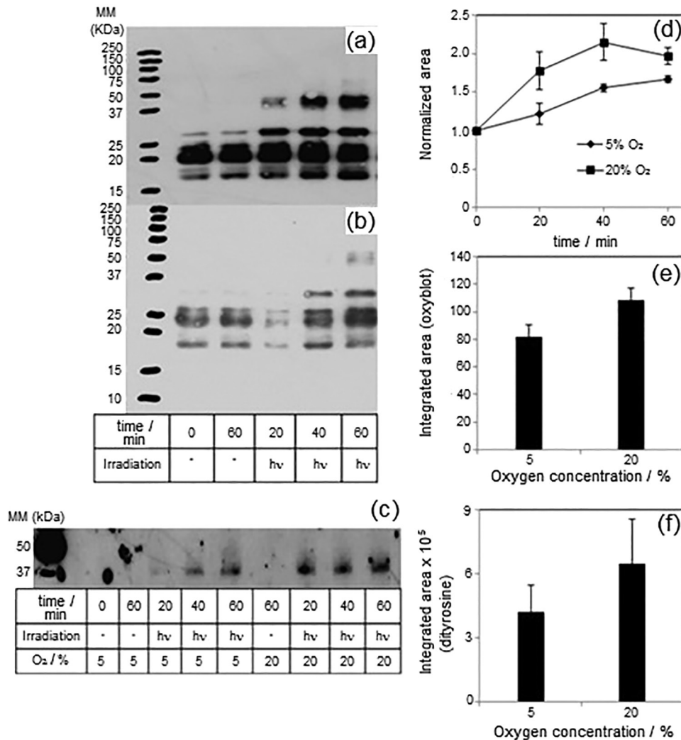
Figure 2. Effect of oxygen in oxidative modifications induced by photosensitized reactions mediated by the major chromophore arising from glucose-derived in eye lens proteins. (a) and (b) show oxyblot analyses when lens proteins were irradiated in the presence of the glucose degradation chromophore (GDC) under constant bubbling with 5 and 20% O 2 ; (c) shows immunochemical detection of dityrosine produced when lens proteins were irradiated in the presence of GDC at 5 and 20% O 2 ; (d) shows the densitometric analyses of oxyblots performed at 5 and 20% O 2 ; (e) and (f) show the integrated area of densitometric analyses of oxyblots and dityrosine blots performed at 5 and 20% O 2 .
